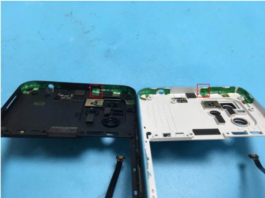
WIFI 5G Antenna
