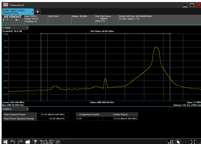
n5_5MHz_15kHz_826.5MHz_DFT-s-OFDM QPSK_RB1@23
