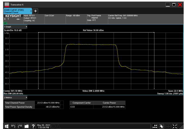
n5_15MHz_15kHz_841.5MHz_DFT-s-OFDM QPSK_RB36@18
