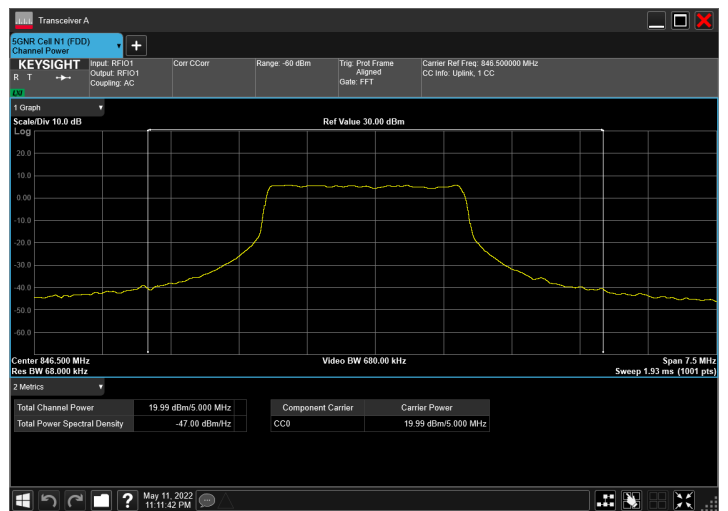
DC_2A_n5A_10MHz|5MHz_15kHz_1905MHz|846.5MHz_QPS K|CP-OFDM 64 QAM_RB12@0|RB13@6
