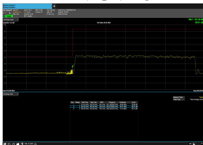
DC_2A_n5A_10MHz|20MHz_15kHz_1880MHz|834MHz_DFT- s-OFDM QPSK_RB0|RB100@0
