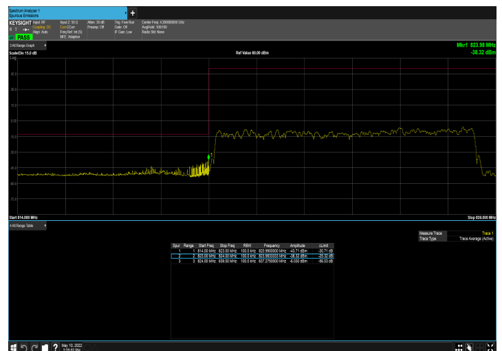
n5_15MHz_15kHz_831.5MHz_DFT-s-OFDM QPSK_RB75@0
