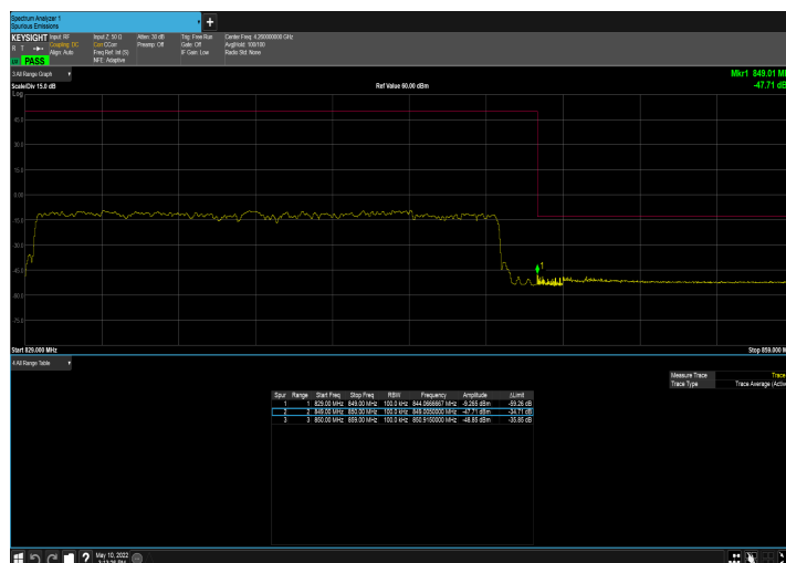
DC_2A_n5A_10MHz|20MHz_15kHz_1880MHz|839MHz_DFT- s-OFDM QPSK_RB0|RB100@0
