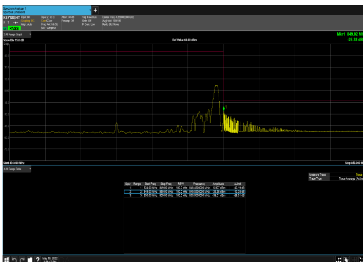
n5_15MHz_15kHz_841.5MHz_DFT-s-OFDM QPSK_RB1@78
