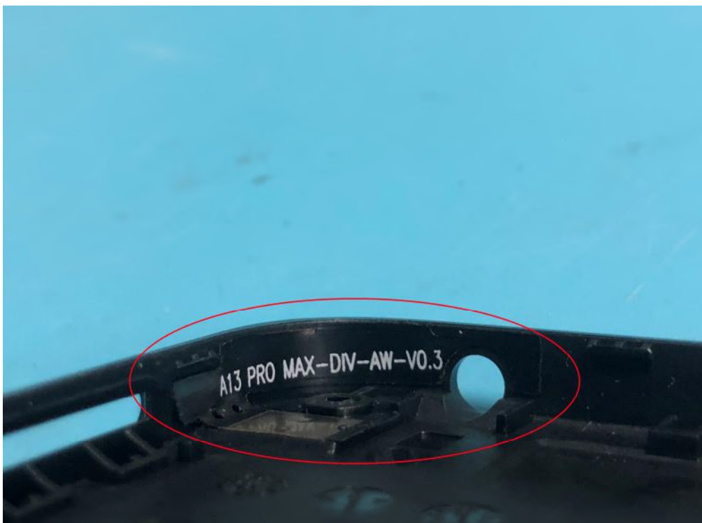
DIV Antenna_GSM850/WCDMA B5/LTE B5/12/13/41 RX, PCS1900/WCDMA B2/LTE B2 TX
