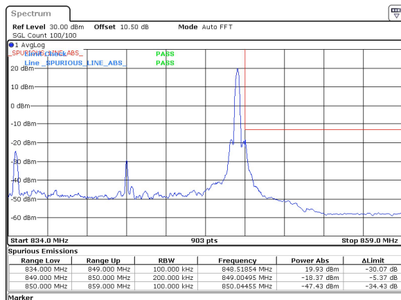
15MHz_15kHz_841.5MHz_DFT-s-OFDM QPSK_RB1@78 -18.37 dBm
