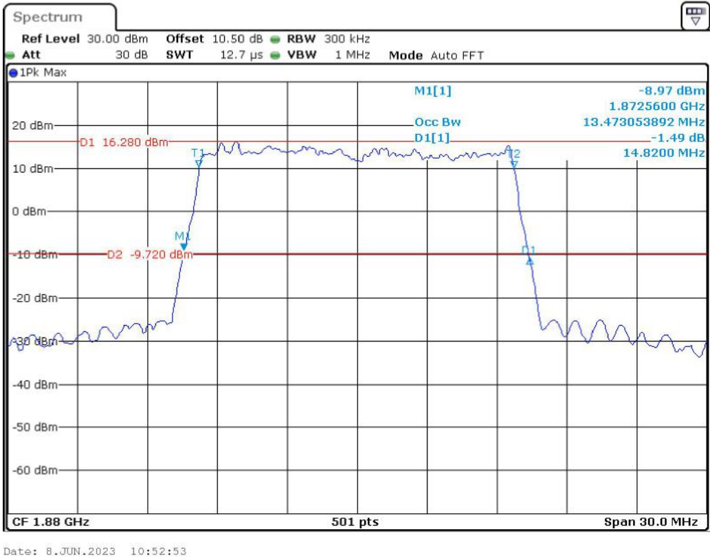
Band 2_15 MHz_Middle_16QAM_RB75#0
