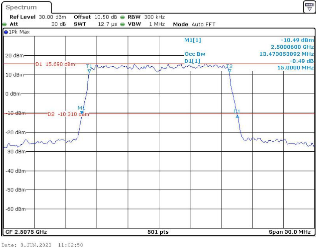
Band 7_15 MHz_Low_QPSK_RB75#0
