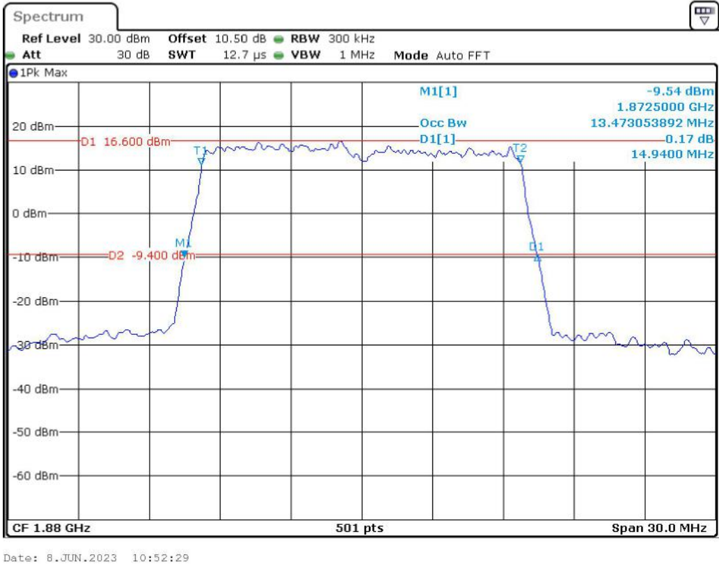
Band 2_15 MHz_Middle_QPSK_RB75#0
