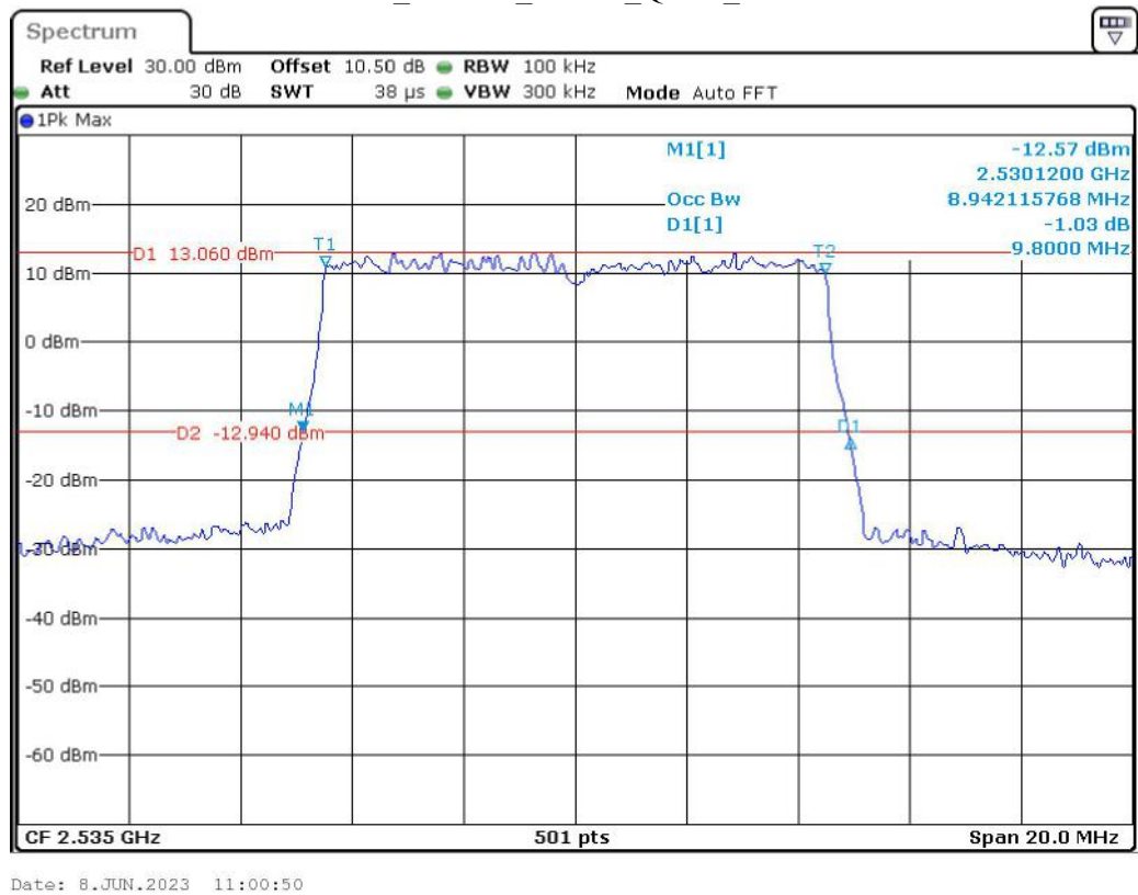
Band 7_10 MHz_Middle_QPSK_RB50#0
