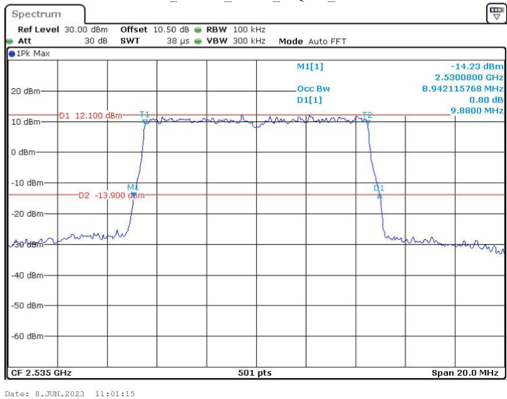
Band 7_10 MHz_Middle_16QAM_RB50#0
