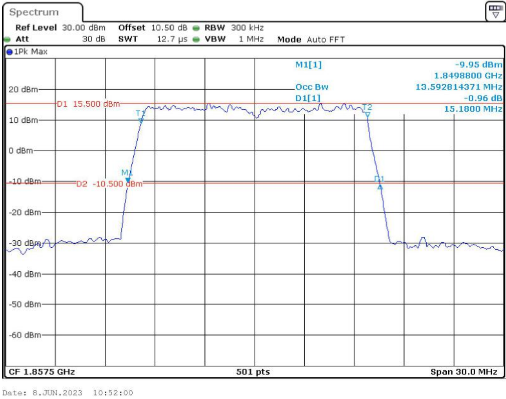
Band 2_15 MHz_Low_16QAM_RB75#0
