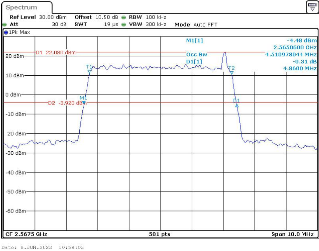
Band 7_5 MHz_High_QPSK_RB25#0
