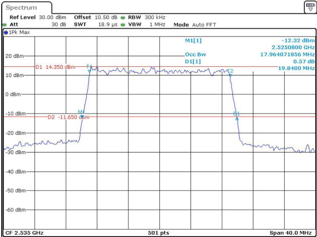
Band 7_20 MHz_Middle_16QAM_RB100#0
