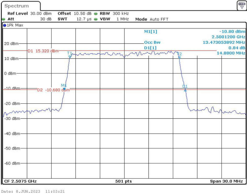
Band 7_15 MHz_Low_16QAM_RB75#0
