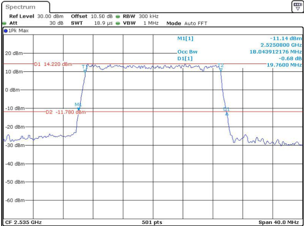
Band 7_20 MHz_Middle_QPSK_RB100#0
