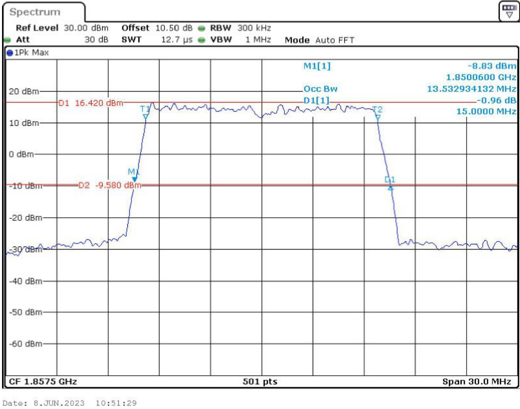
Band 2_15 MHz_Low_QPSK_RB75#0
