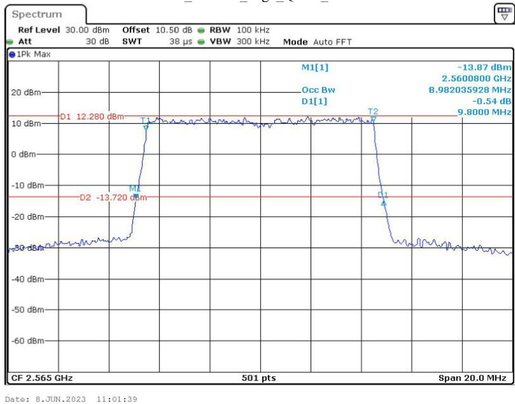
Band 7_10 MHz_High_QPSK_RB50#0
