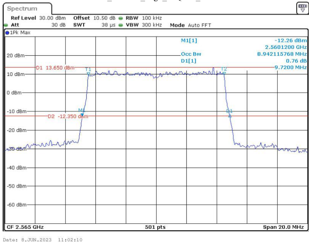
Band 7_10 MHz_High_16QAM_RB50#0
