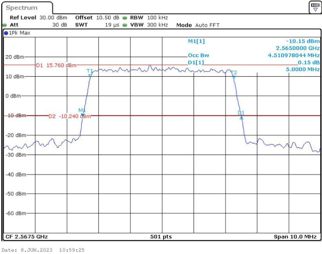
Band 7_5 MHz_High_16QAM_RB25#0
