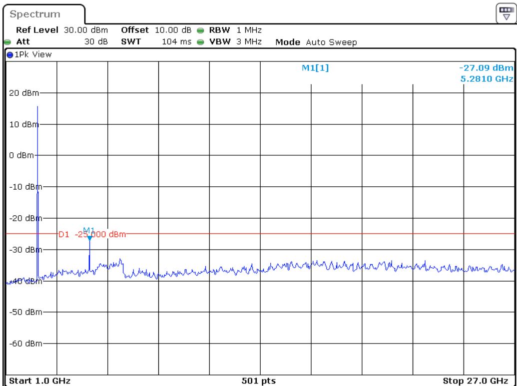
Band 41_5 MHz_Low_QPSK_RB25#0_2(1GHz-27GHz)
