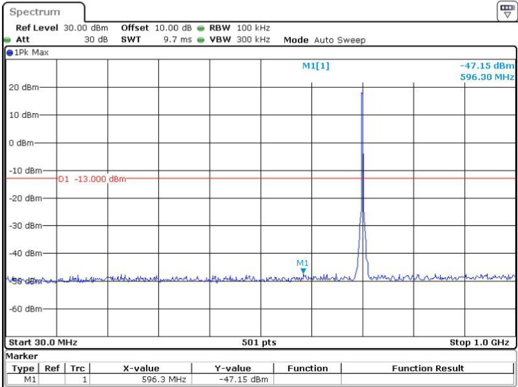
Band 12_3 MHz_Middle_QPSK_RB15#0_1(30MHz-1GHz)
