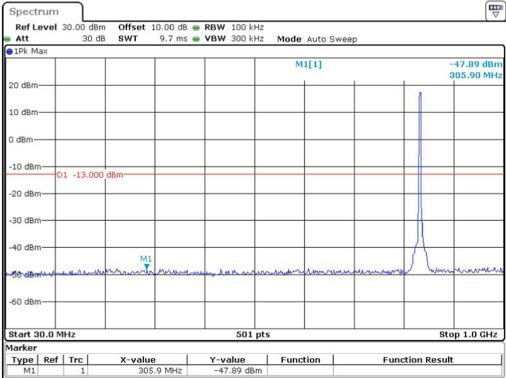
Band 5_3 MHz_Middle_QPSK_RB15#0_1(30MHz-1GHz)
