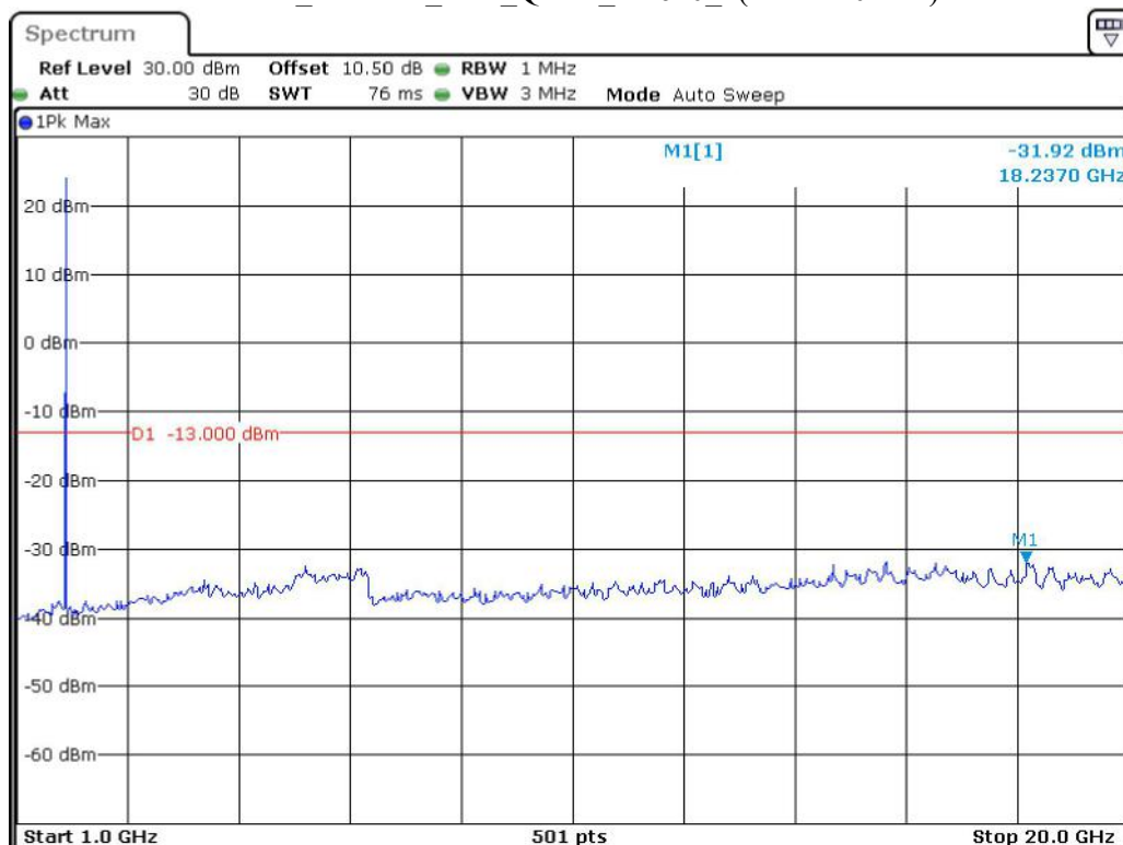
Band 2_1.4 MHz_Low_QPSK_RB6#0_2(1GHz-20GHz)
