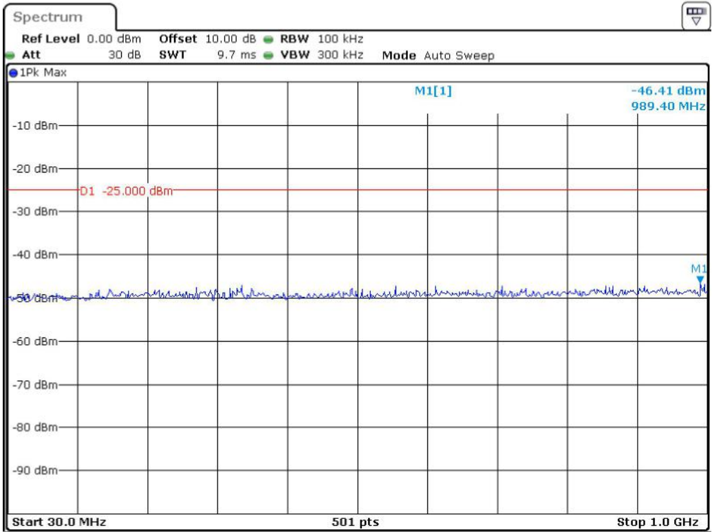
Band 41_5 MHz_Low_QPSK_RB25#0_1(30MHz-1GHz)
