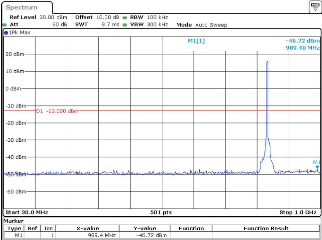
Band 5_5 MHz_Middle_QPSK_RB25#0_1(30MHz-1GHz)
