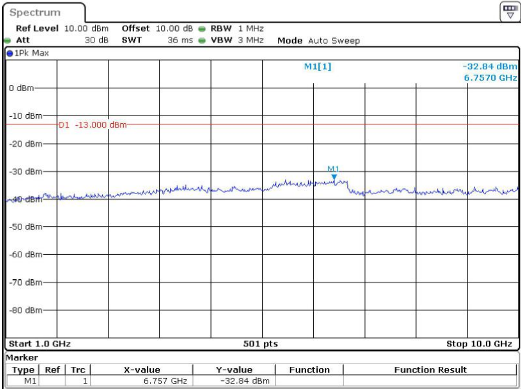
Band 5_5 MHz_Middle_QPSK_RB25#0_2(1GHz-10GHz)
