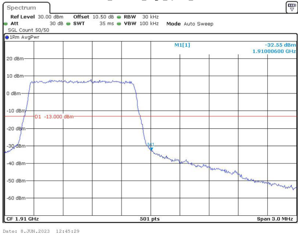
Band 2_1.4 MHz_High_QPSK_RB6#0
