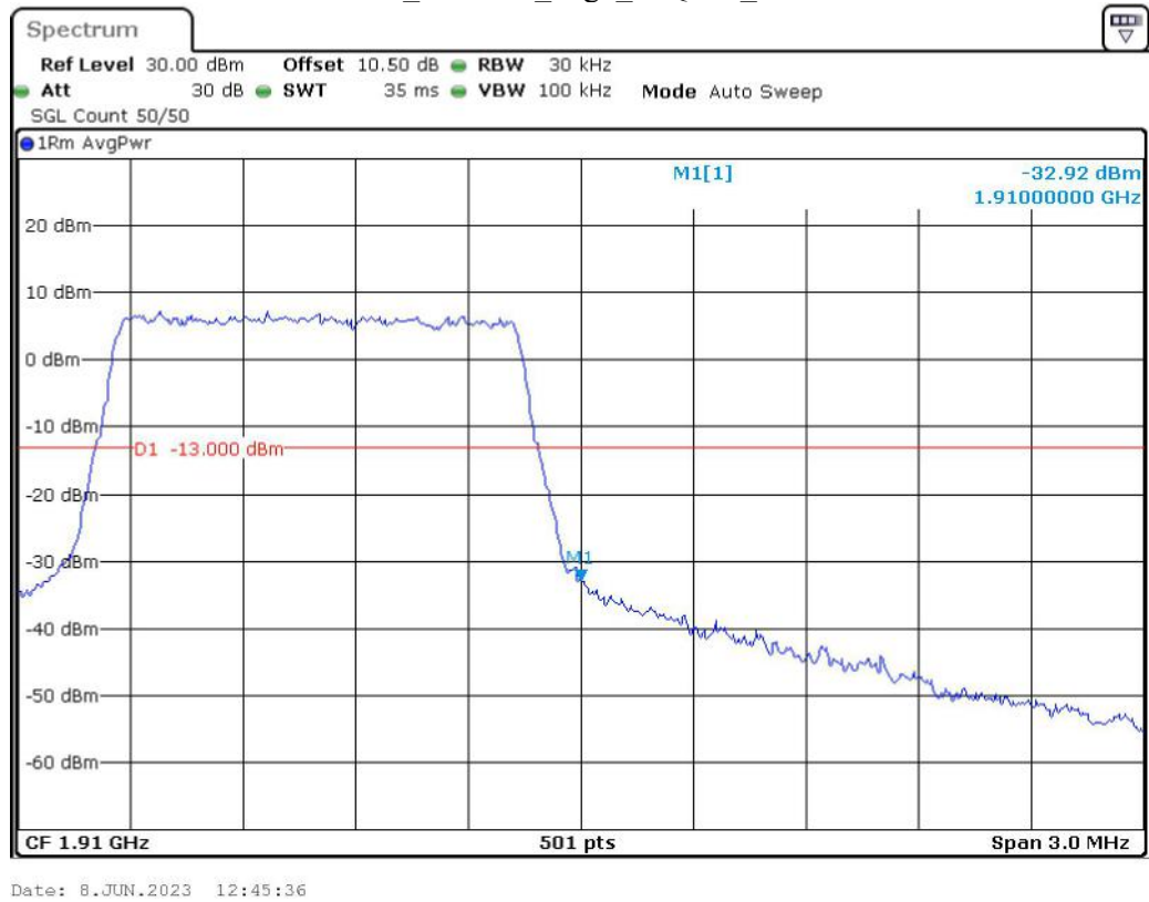
Band 2_1.4 MHz_High_16QAM_RB6#0
