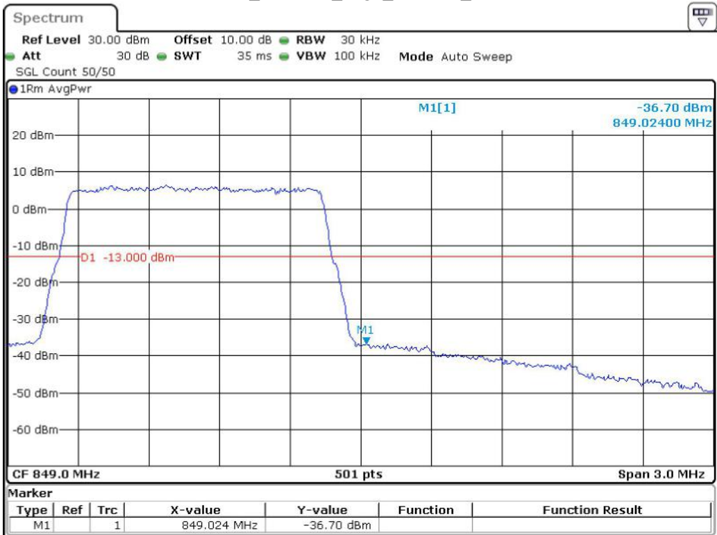
Band 5_1.4 MHz_High_16QAM_RB6#0
