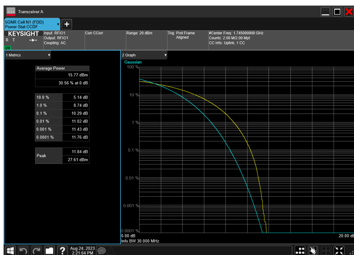
n66_30MHz_15kHz_1745MHz_CP-OFDM QPSK_RB160@0
