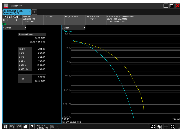
n66_30MHz_15kHz_1745MHz_CP-OFDM 256 QAM_RB160@0
