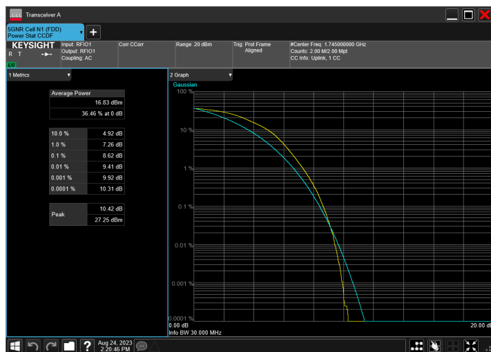
n66_30MHz_15kHz_1745MHz_DFT-s-OFDM 16 QAM_RB160@0
