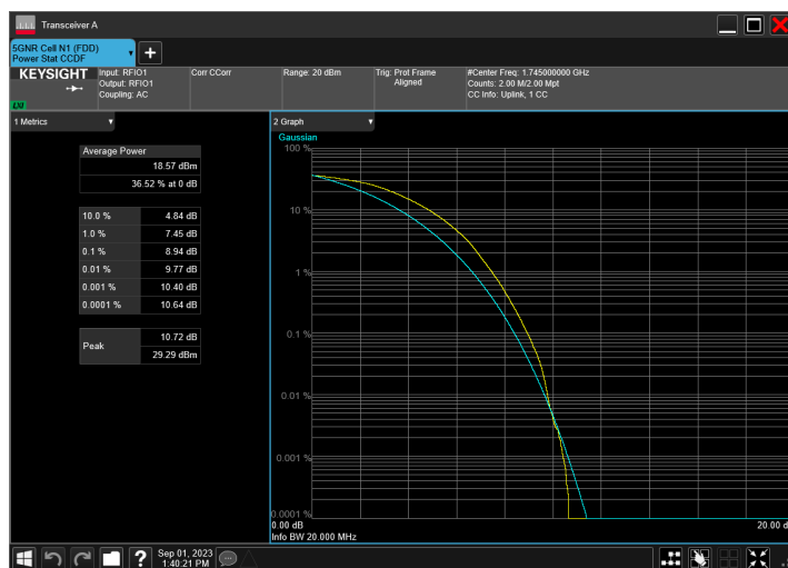
n66_20MHz_15kHz_1745MHz_DFT-s-OFDM 64 QAM_RB100@0
