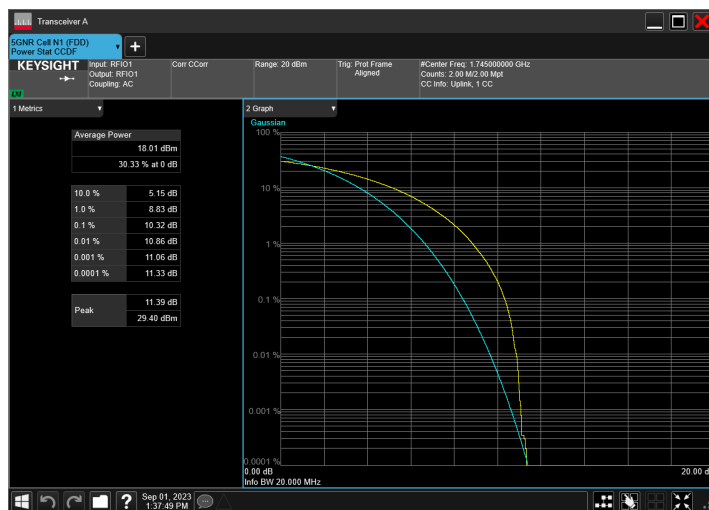
n66_15MHz_15kHz_1745MHz_CP-OFDM 16 QAM_RB79@0
