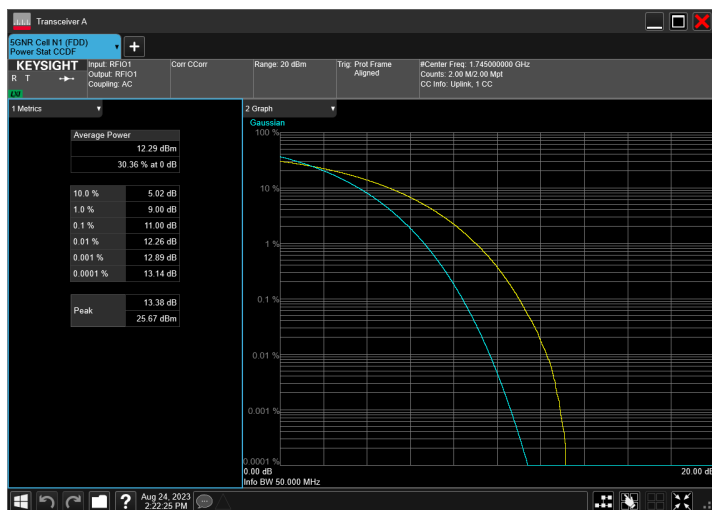
n66_40MHz_15kHz_1745MHz_CP-OFDM 256 QAM_RB216@0
