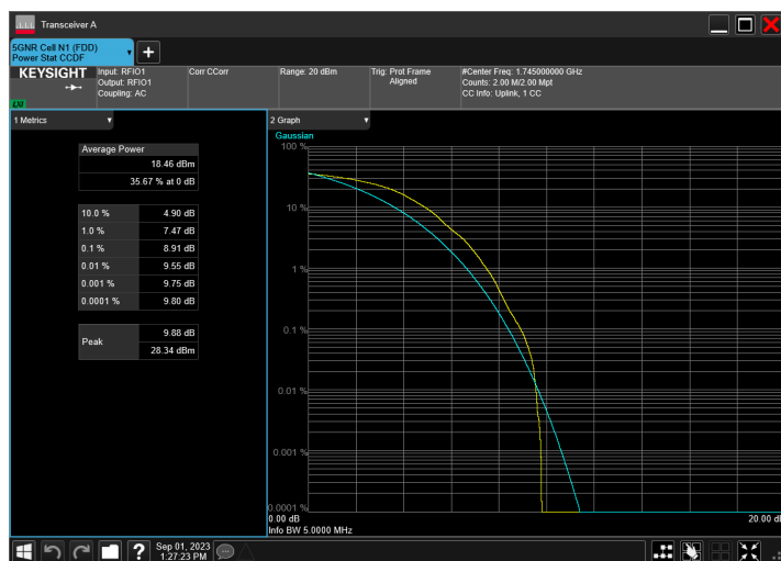
n66_5MHz_15kHz_1745MHz_DFT-s-OFDM 64 QAM_RB25@0
