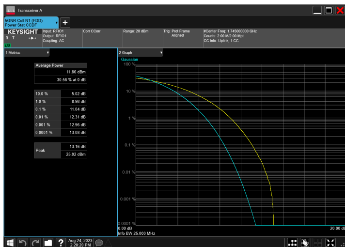
n66_25MHz_15kHz_1745MHz_CP-OFDM 256 QAM_RB133@0
