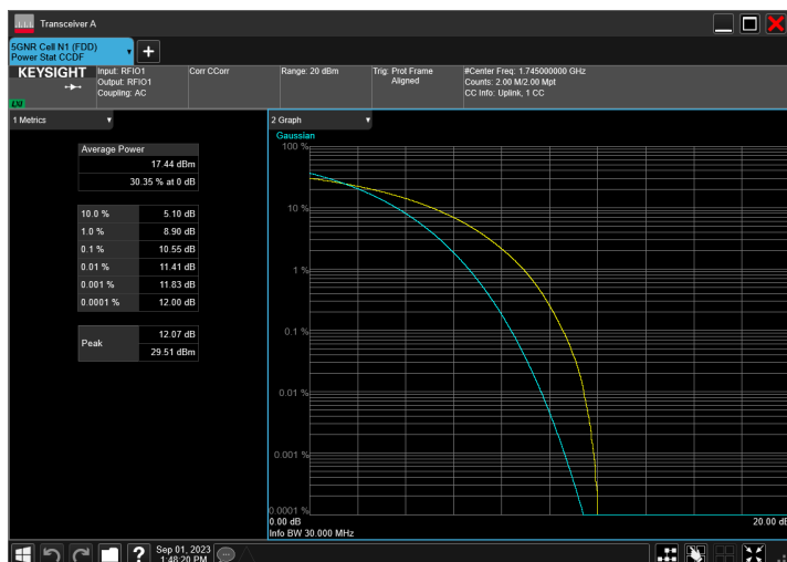
n66_30MHz_15kHz_1745MHz_CP-OFDM 64 QAM_RB160@0
