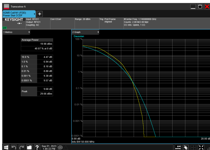
n66_40MHz_15kHz_1745MHz_DFT-s-OFDM QPSK_RB216@0
