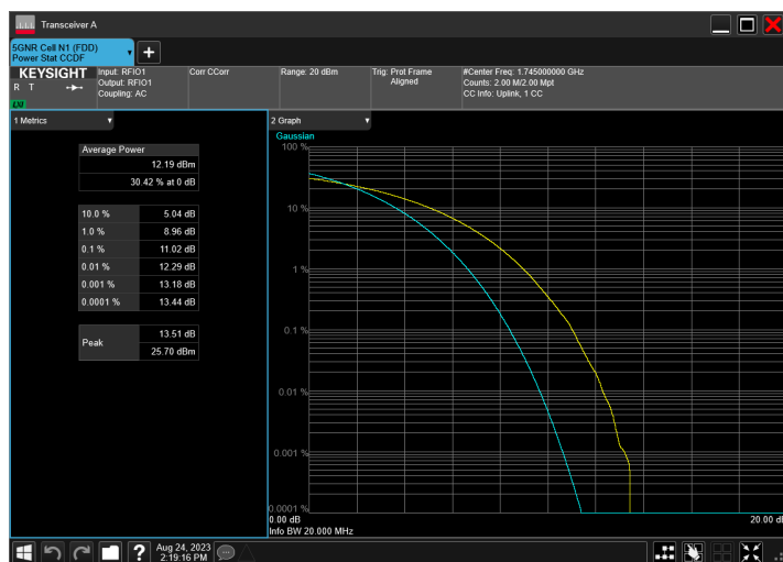
n66_20MHz_15kHz_1745MHz_CP-OFDM 256 QAM_RB106@0
