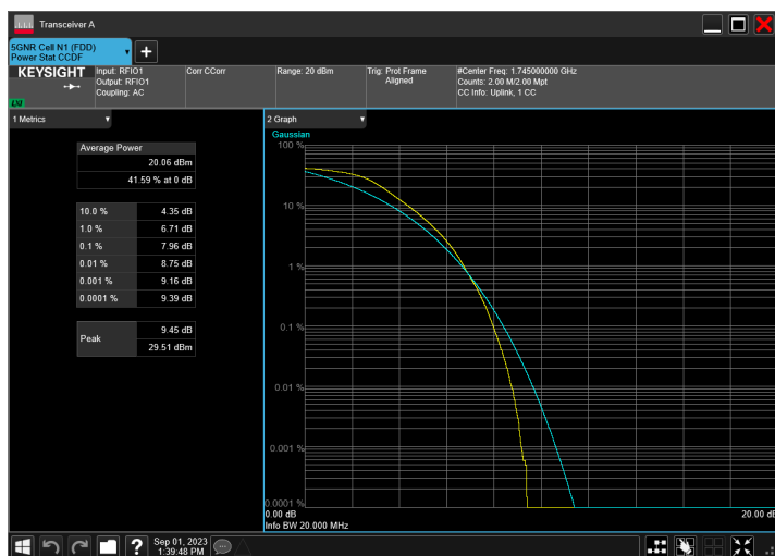
n66_20MHz_15kHz_1745MHz_DFT-s-OFDM QPSK_RB100@0
