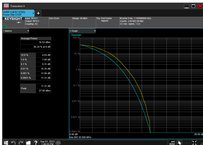
n66_20MHz_15kHz_1745MHz_DFT-s-OFDM 256 QAM_RB100@0
