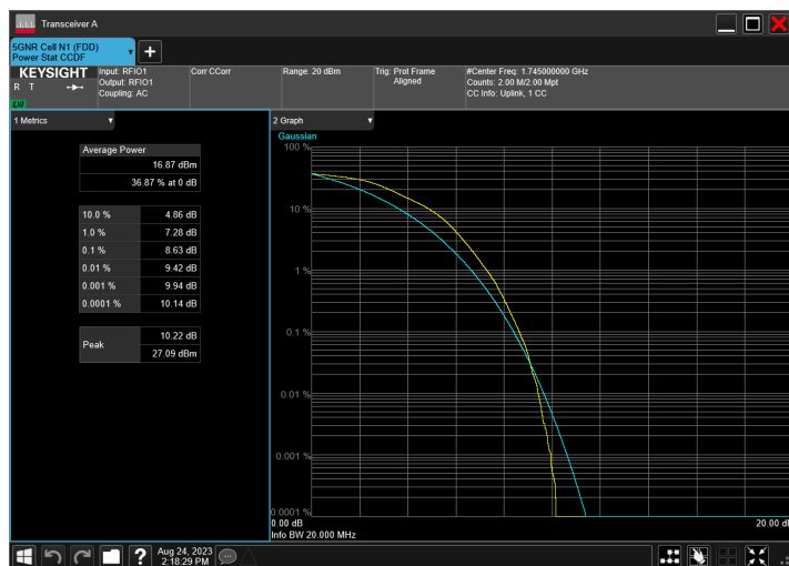
n66_20MHz_15kHz_1745MHz_DFT-s-OFDM 16 QAM_RB100@0
