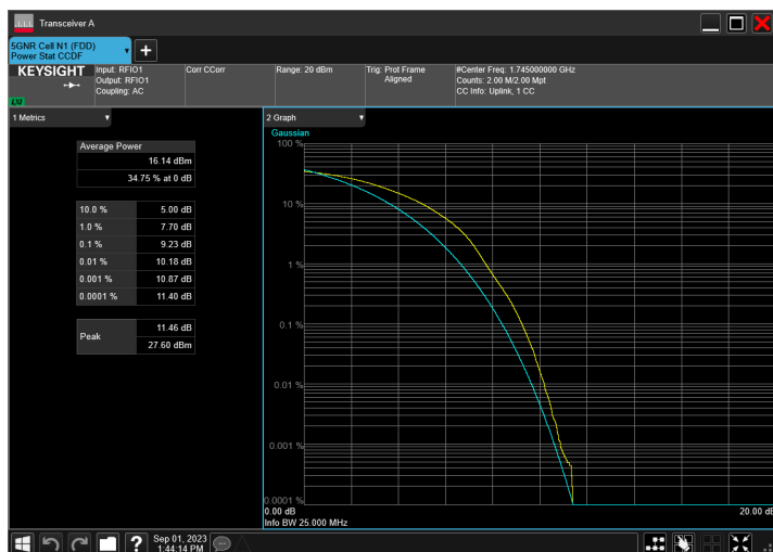
n66_25MHz_15kHz_1745MHz_DFT-s-OFDM 256 QAM_RB128@0
