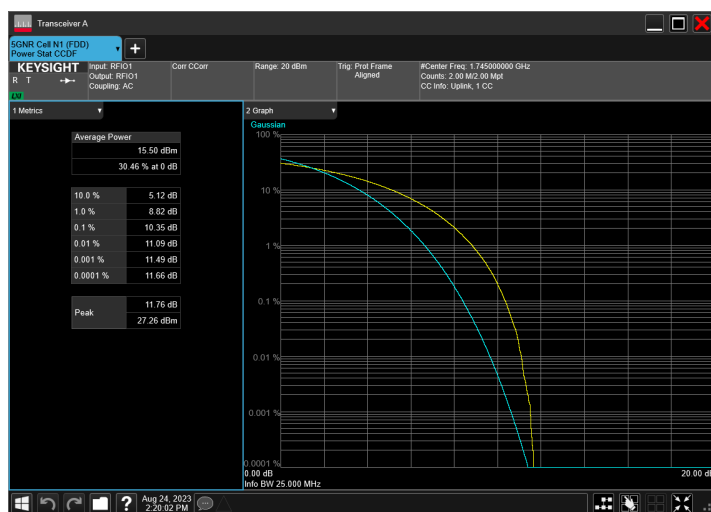
n66_25MHz_15kHz_1745MHz_CP-OFDM QPSK_RB133@0
