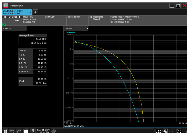
n66_25MHz_15kHz_1745MHz_CP-OFDM 64 QAM_RB133@0
