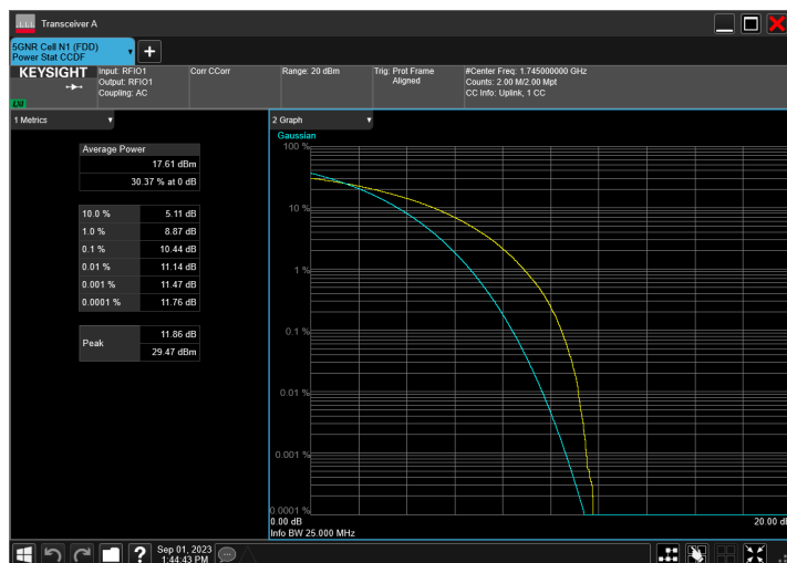
n66_25MHz_15kHz_1745MHz_CP-OFDM 16 QAM_RB133@0
