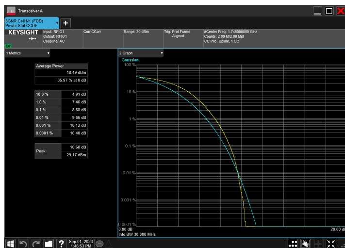
n66_30MHz_15kHz_1745MHz_DFT-s-OFDM 64 QAM_RB160@0
