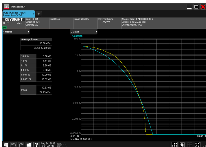
n66_40MHz_15kHz_1745MHz_DFT-s-OFDM 16 QAM_RB216@0
