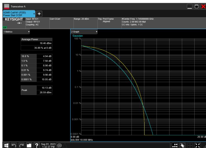
n66_10MHz_15kHz_1745MHz_DFT-s-OFDM 64 QAM_RB50@0
