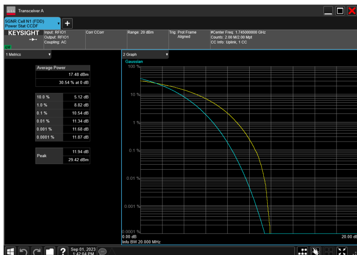
n66_20MHz_15kHz_1745MHz_CP-OFDM 64 QAM_RB106@0
