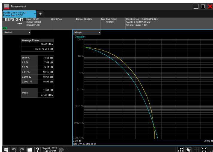
n66_30MHz_15kHz_1745MHz_DFT-s-OFDM 256 QAM_RB160@0
