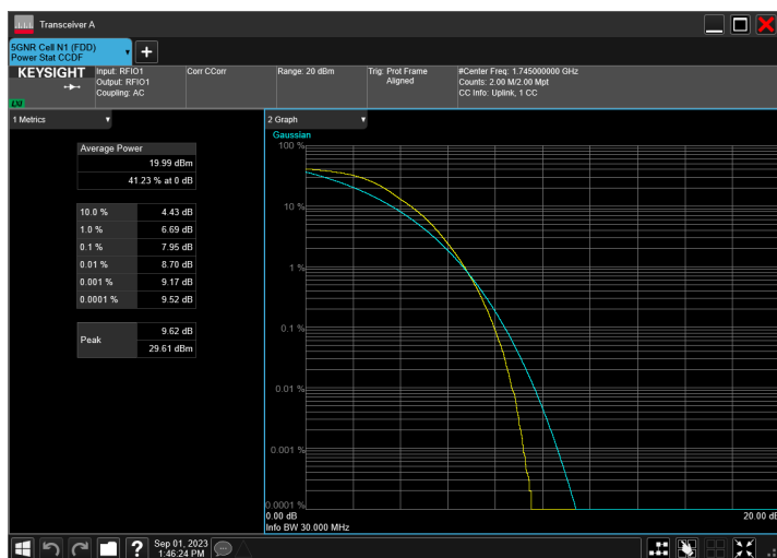
n66_30MHz_15kHz_1745MHz_DFT-s-OFDM QPSK_RB160@0
