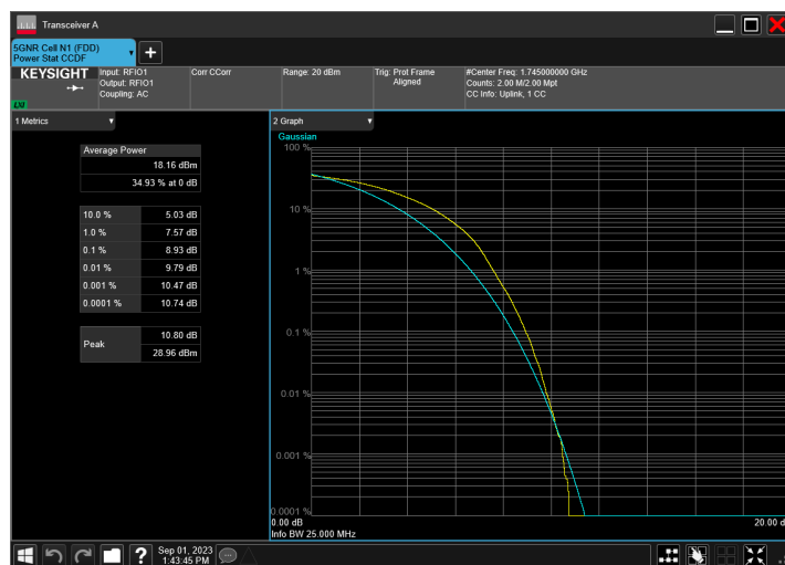
n66_25MHz_15kHz_1745MHz_DFT-s-OFDM 64 QAM_RB128@0
