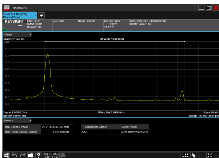
n66_40MHz_15kHz_1745MHz_DFT-s-OFDM QPSK_RB1@1
