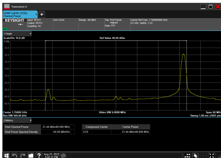
n66_40MHz_15kHz_1760MHz_DFT-s-OFDM QPSK_RB1@214
