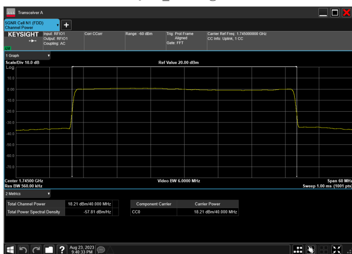
n66_40MHz_15kHz_1745MHz_CP-OFDM 64 QAM_RB216@0
