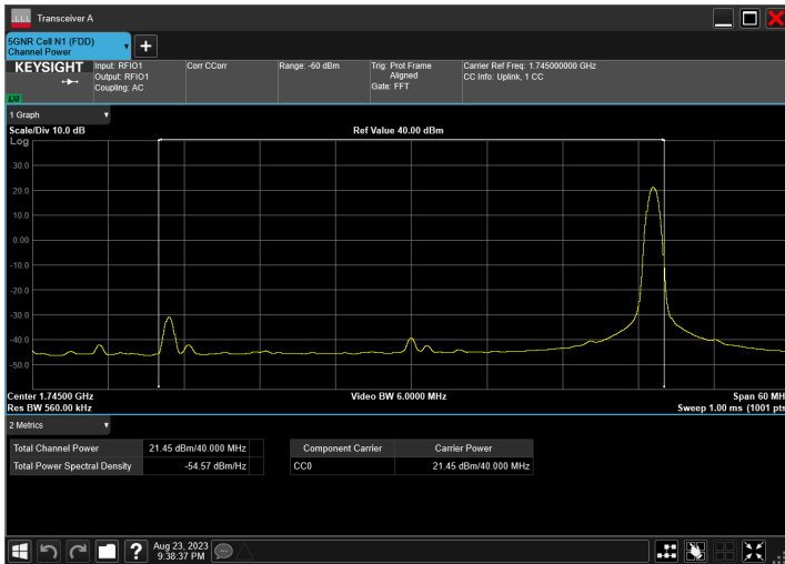
n66_40MHz_15kHz_1745MHz_DFT-s-OFDM QPSK_RB1@214
