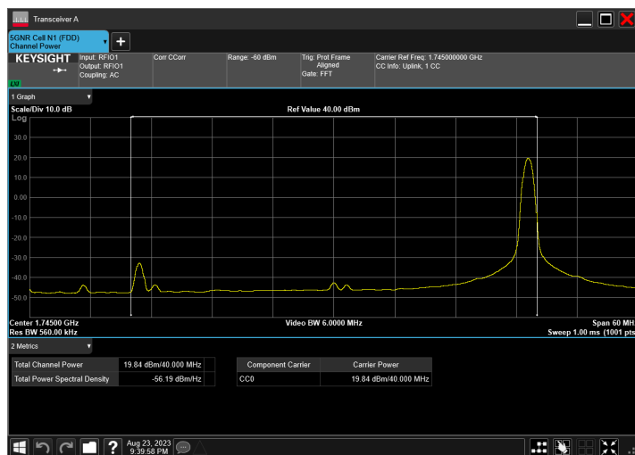
n66_40MHz_15kHz_1745MHz_CP-OFDM 16 QAM_RB216@0
