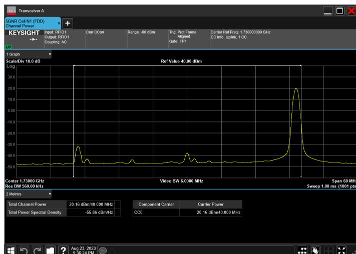
n66_40MHz_15kHz_1730MHz_CP-OFDM 16 QAM_RB216@0
