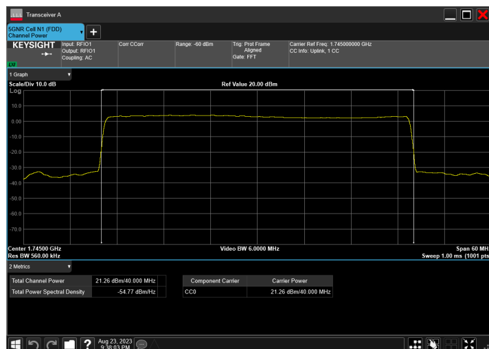
n66_40MHz_15kHz_1745MHz_DFT-s-OFDM PI/2 BPSK_RB216@0
