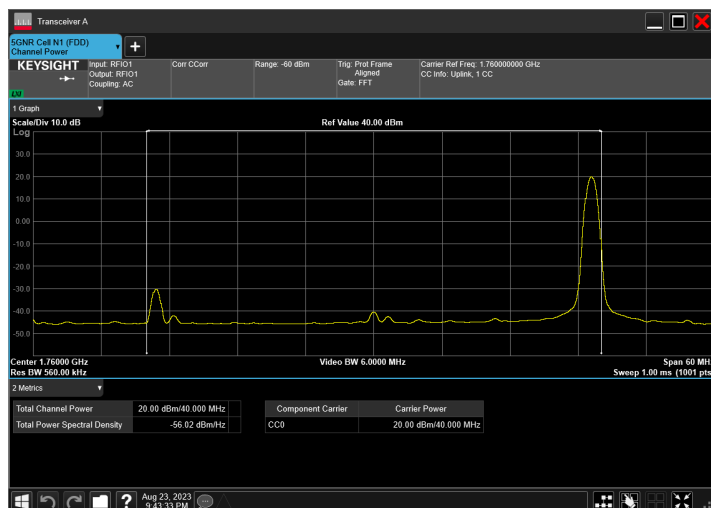
n66_40MHz_15kHz_1760MHz_CP-OFDM 16 QAM_RB216@0
