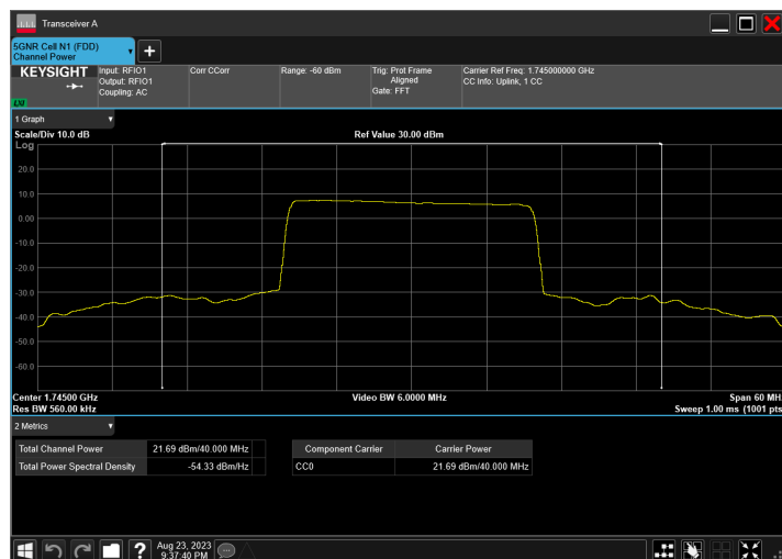
n66_40MHz_15kHz_1745MHz_DFT-s-OFDM PI/2 BPSK_RB108@54
