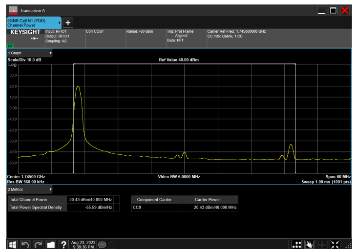
n66_40MHz_15kHz_1745MHz_CP-OFDM QPSK_RB1@1
