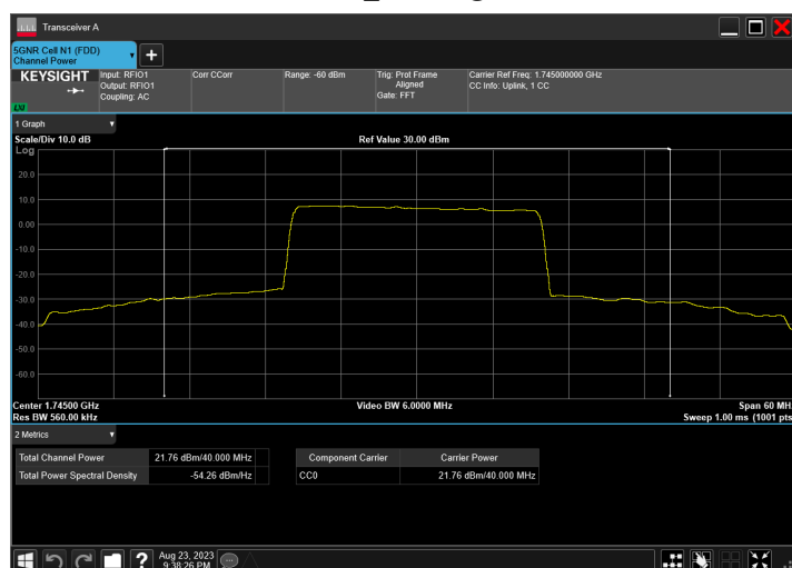
n66_40MHz_15kHz_1745MHz_DFT-s-OFDM QPSK_RB108@54
