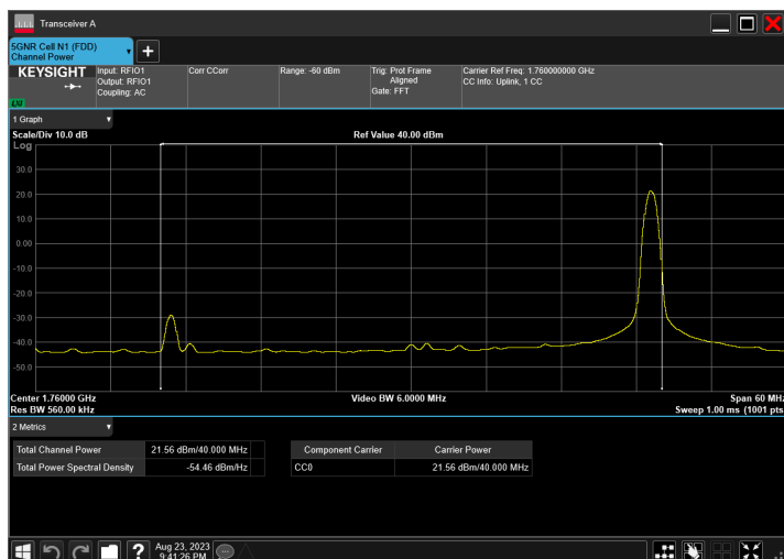
n66_40MHz_15kHz_1760MHz_DFT-s-OFDM PI/2 BPSK_RB1@214
