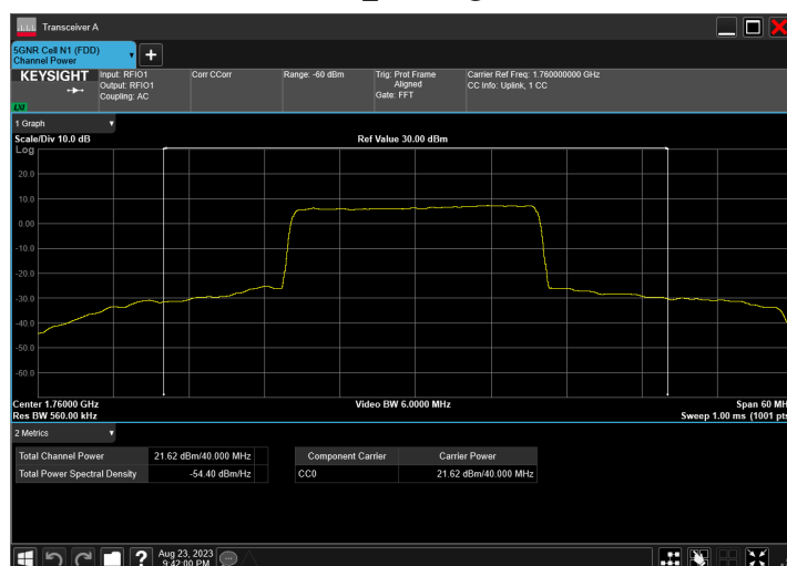
n66_40MHz_15kHz_1760MHz_DFT-s-OFDM QPSK_RB108@54
