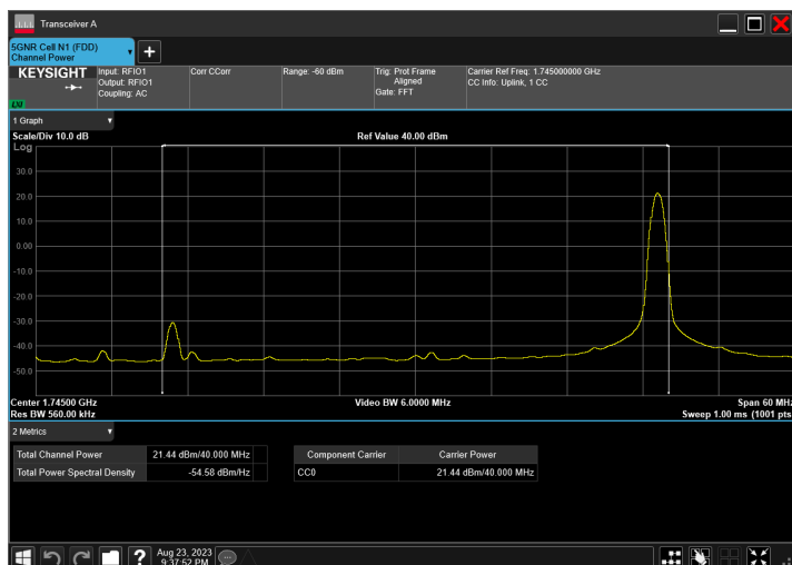
n66_40MHz_15kHz_1745MHz_DFT-s-OFDM PI/2 BPSK_RB1@214
