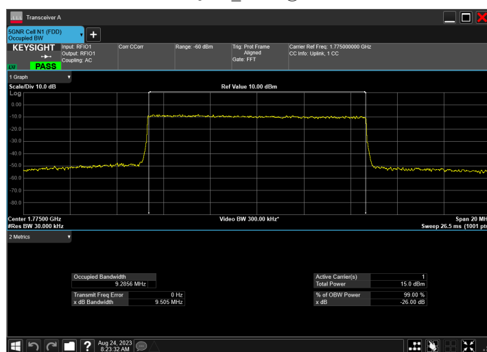
n66_10MHz_15kHz_1775MHz_CP-OFDM 256 QAM_RB52@0
