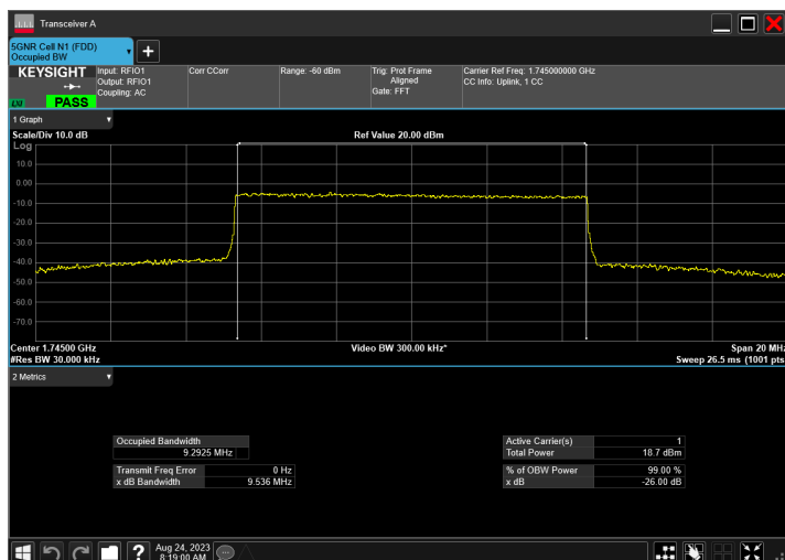
n66_10MHz_15kHz_1745MHz_CP-OFDM 256 QAM_RB52@0
