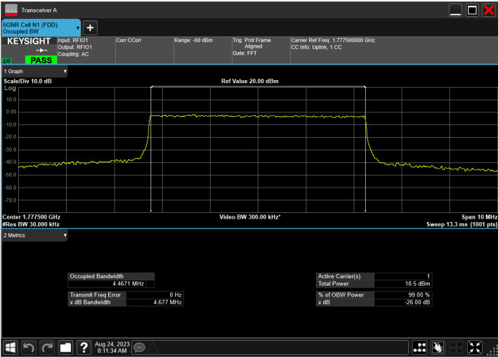
n66_5MHz_15kHz_1777.5MHz_CP-OFDM 256 QAM_RB25@0
