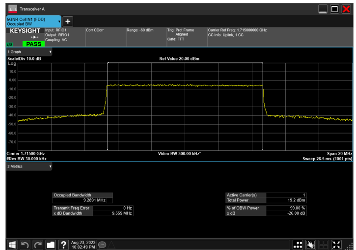
n66_10MHz_15kHz_1715MHz_CP-OFDM 256 QAM_RB52@0
