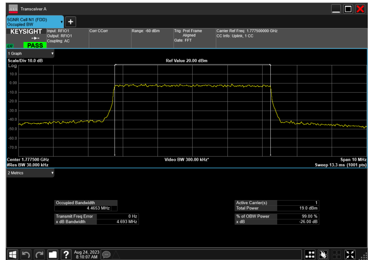
n66_5MHz_15kHz_1777.5MHz_DFT-s-OFDM 64 QAM_RB25@0
