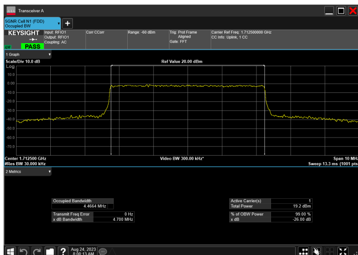
n66_5MHz_15kHz_1712.5MHz_CP-OFDM 256 QAM_RB25@0
