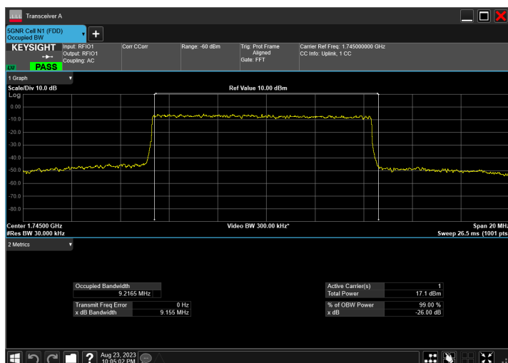
n66_10MHz_15kHz_1745MHz_DFT-s-OFDM 256 QAM_RB50@0
