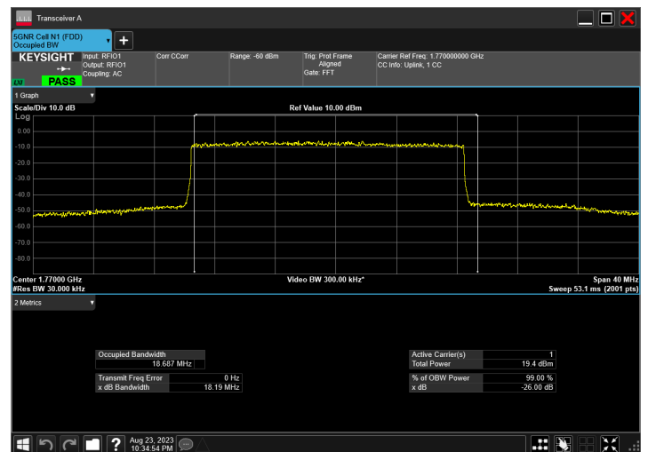
n66_20MHz_15kHz_1770MHz_DFT-s-OFDM 16 QAM_RB100@0
