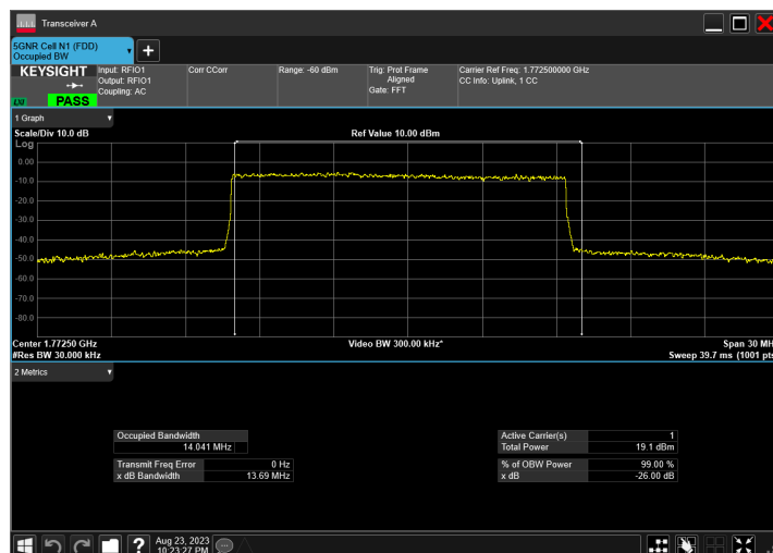
n66_15MHz_15kHz_1772.5MHz_DFT-s-OFDM 64 QAM_RB75@0
