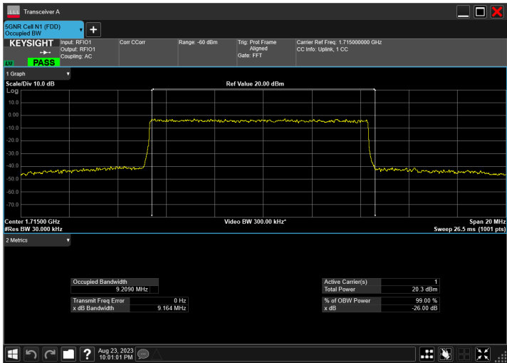
n66_10MHz_15kHz_1715MHz_DFT-s-OFDM 16 QAM_RB50@0
