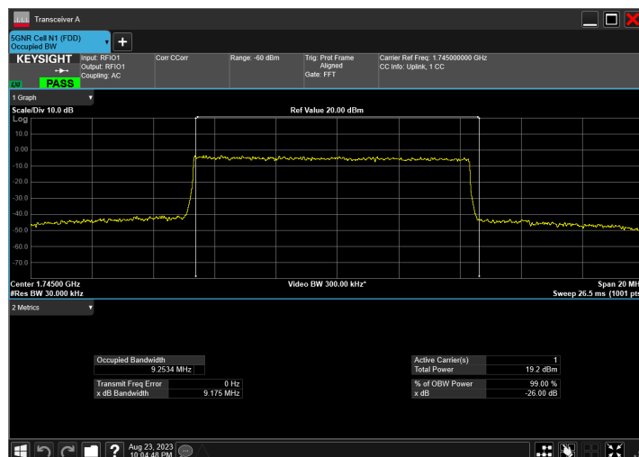
n66_10MHz_15kHz_1745MHz_DFT-s-OFDM 64 QAM_RB50@0
