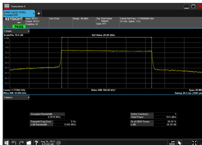
n66_10MHz_15kHz_1775MHz_CP-OFDM 256 QAM_RB52@0
