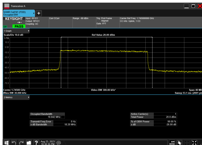
n66_20MHz_15kHz_1745MHz_DFT-s-OFDM QPSK_RB100@0
