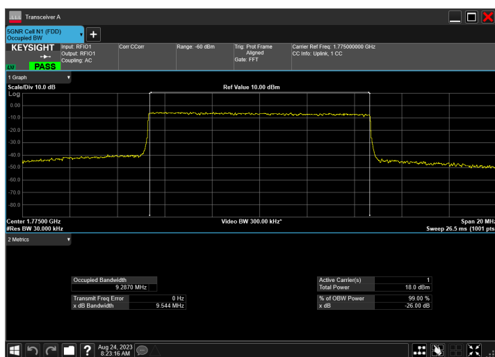
n66_10MHz_15kHz_1775MHz_CP-OFDM 64 QAM_RB52@0
