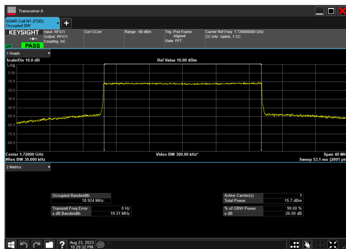
n66_20MHz_15kHz_1720MHz_CP-OFDM 256 QAM_RB106@0
