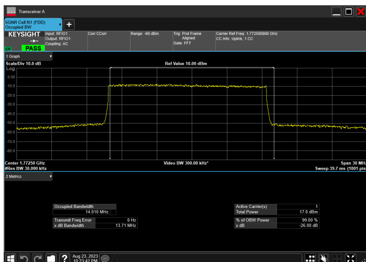
n66_15MHz_15kHz_1772.5MHz_DFT-s-OFDM 256 QAM_RB75@0
