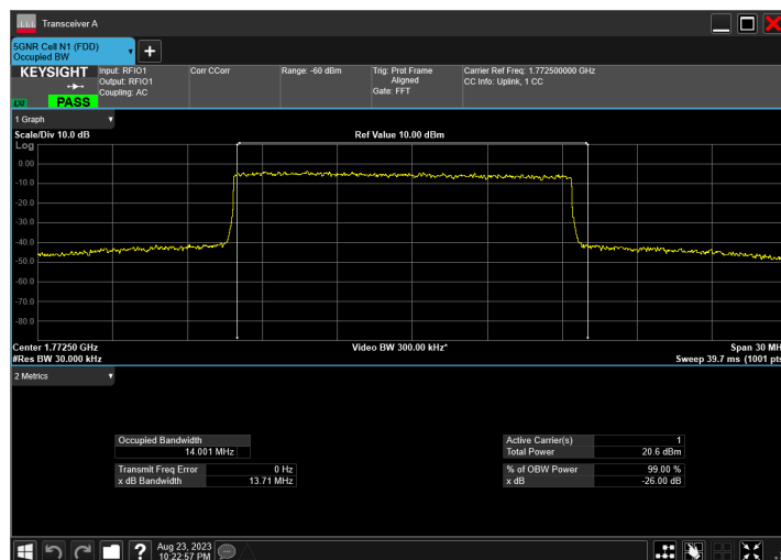
n66_15MHz_15kHz_1772.5MHz_DFT-s-OFDM QPSK_RB75@0
