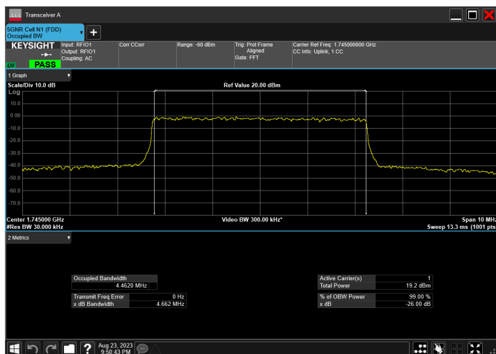
n66_5MHz_15kHz_1745MHz_DFT-s-OFDM 64 QAM_RB25@0
