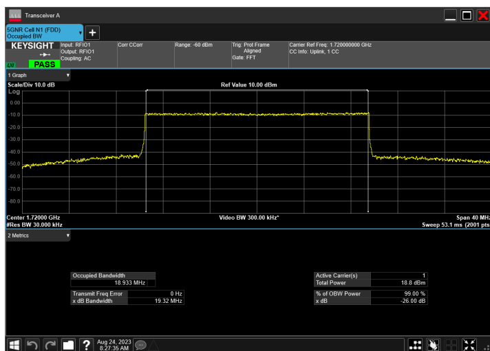
n66_20MHz_15kHz_1720MHz_CP-OFDM 64 QAM_RB106@0
