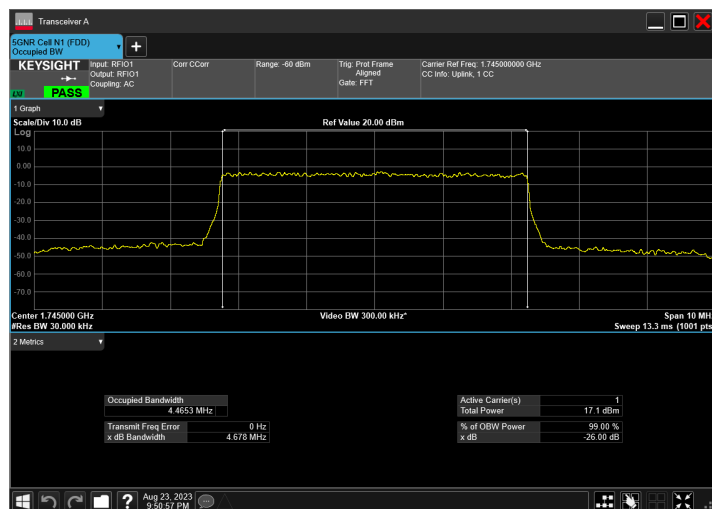
n66_5MHz_15kHz_1745MHz_DFT-s-OFDM 256 QAM_RB25@0
