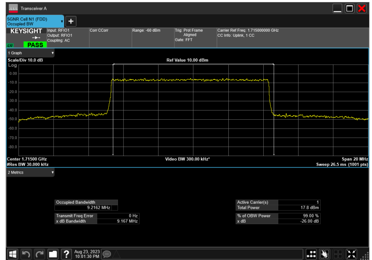
n66_10MHz_15kHz_1715MHz_CP-OFDM 16 QAM_RB52@0
