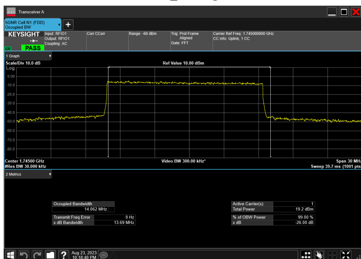
n66_15MHz_15kHz_1745MHz_DFT-s-OFDM 64 QAM_RB75@0
