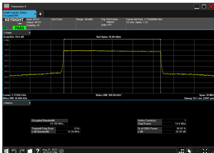
n66_15MHz_15kHz_1772.5MHz_CP-OFDM 256 QAM_RB79@0
