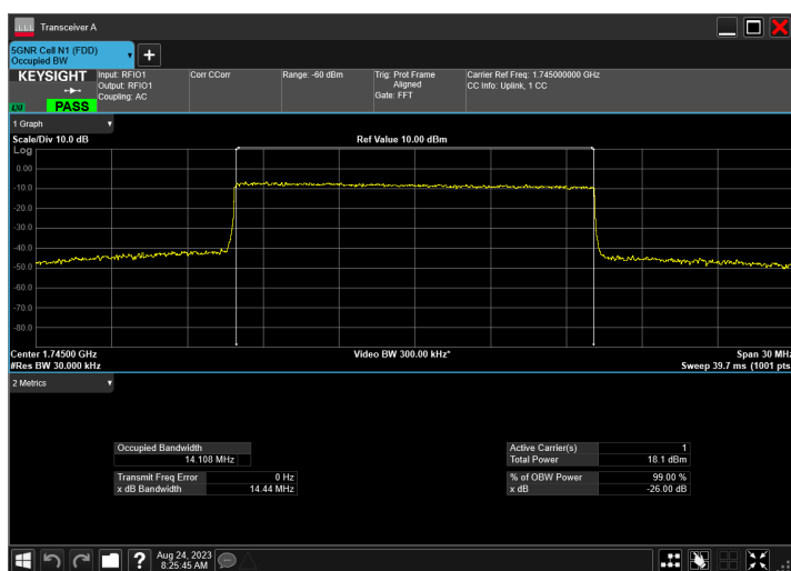
n66_15MHz_15kHz_1745MHz_CP-OFDM 64 QAM_RB79@0
