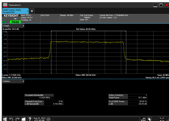
n66_10MHz_15kHz_1775MHz_DFT-s-OFDM 64 QAM_RB50@0
