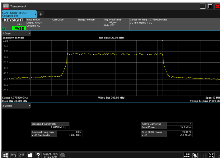
n66_5MHz_15kHz_1777.5MHz_DFT-s-OFDM 256 QAM_RB25@0
