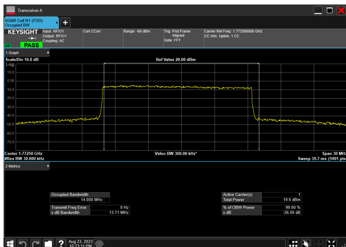
n66_15MHz_15kHz_1772.5MHz_DFT-s-OFDM 16 QAM_RB75@0
