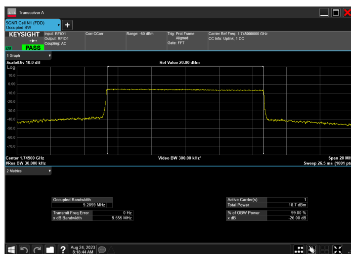
n66_10MHz_15kHz_1745MHz_CP-OFDM QPSK_RB52@0
