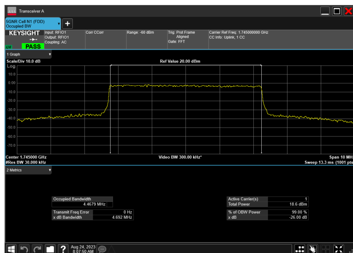
n66_5MHz_15kHz_1745MHz_CP-OFDM 256 QAM_RB25@0
