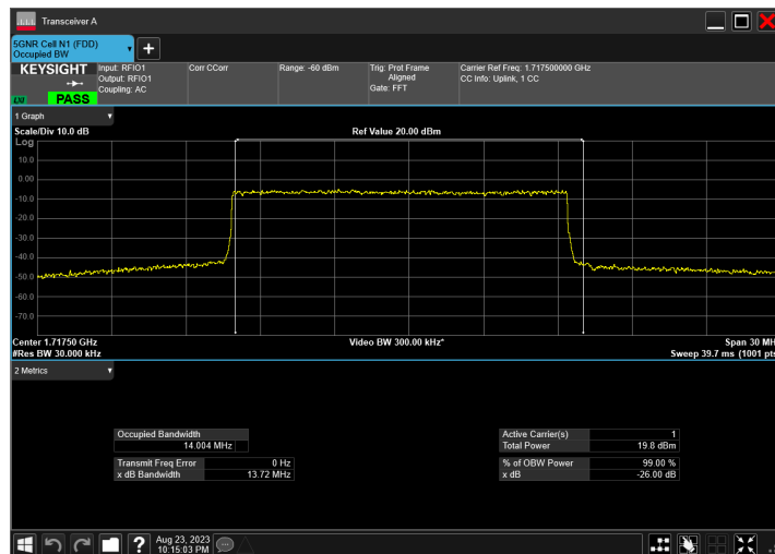
n66_15MHz_15kHz_1717.5MHz_DFT-s-OFDM 64 QAM_RB75@0
