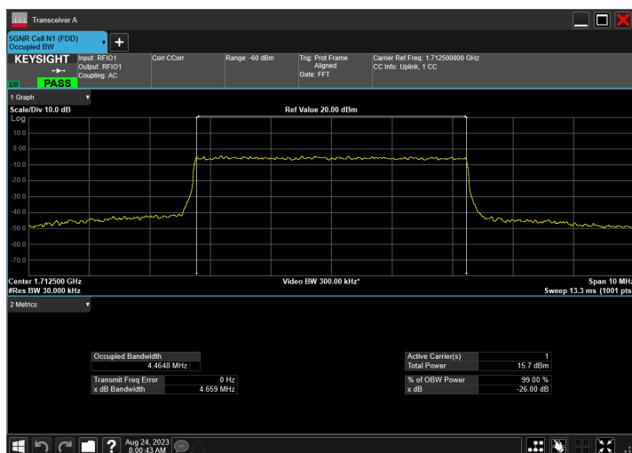
n66_5MHz_15kHz_1712.5MHz_CP-OFDM 256 QAM_RB25@0
