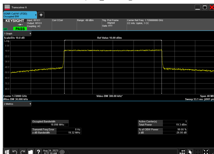
n66_20MHz_15kHz_1720MHz_CP-OFDM 16 QAM_RB106@0
