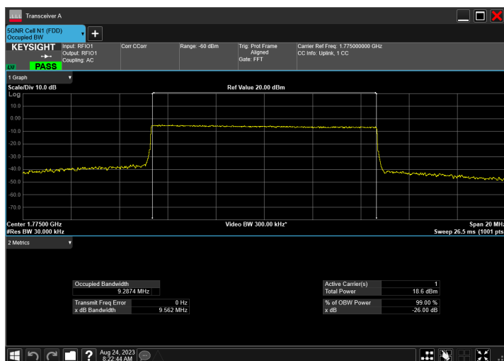
n66_10MHz_15kHz_1775MHz_CP-OFDM 64 QAM_RB52@0
