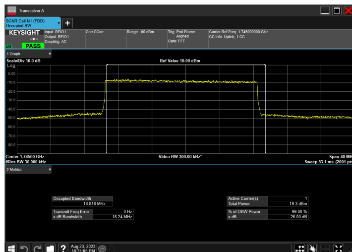
n66_20MHz_15kHz_1745MHz_DFT-s-OFDM 64 QAM_RB100@0
