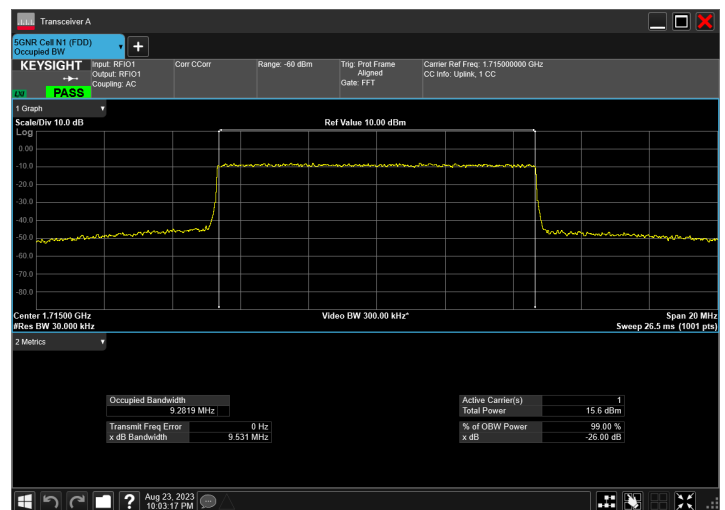
n66_10MHz_15kHz_1715MHz_CP-OFDM 256 QAM_RB52@0
