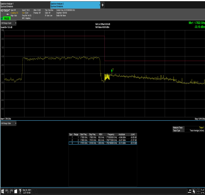
n66_25MHz_15kHz_1767.5MHz_DFT-s-OFDM QPSK_RB128@0
