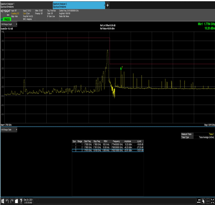
n66_25MHz_15kHz_1767.5MHz_DFT-s-OFDM QPSK_RB1@132
