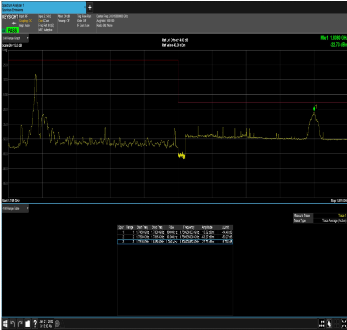
n66_30MHz_15kHz_1765MHz_DFT-s-OFDM QPSK_RB1@0
