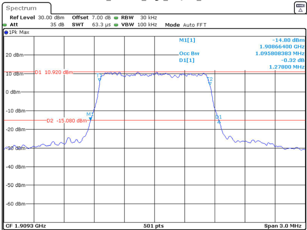
Band 2_1.4 MHz_High_16QAM_RB6#0
