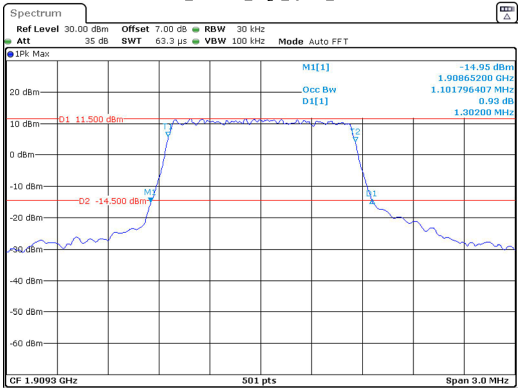
Band 2_1.4 MHz_High_QPSK_RB6#0
