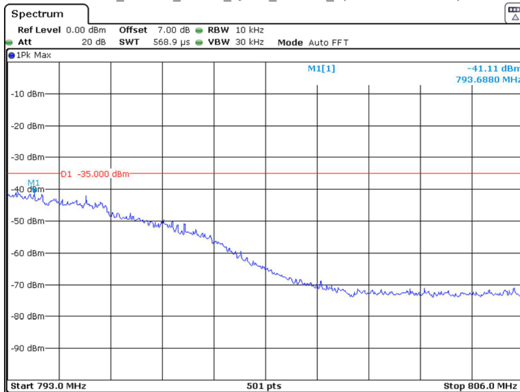
Band 13_10 MHz_Middle_QPSK_RB50#0_4(793MHz-806MHz)
