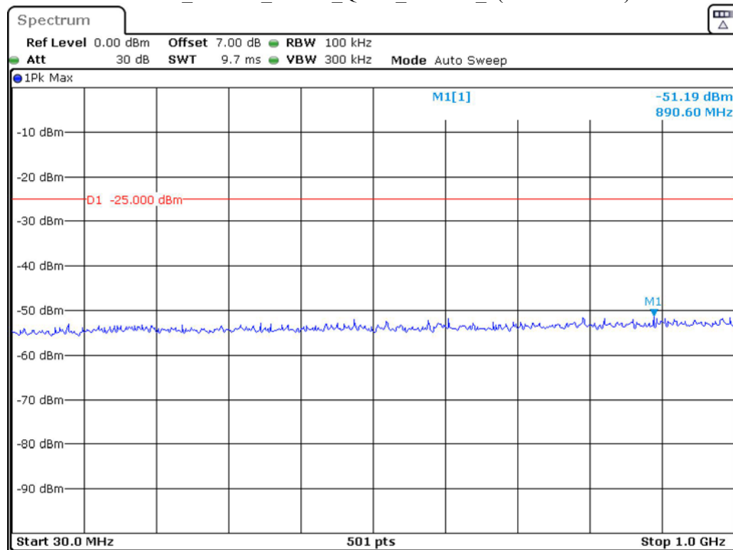
Band 41_10 MHz_Middle_QPSK_RB50#0_1(30MHz-1GHz)
