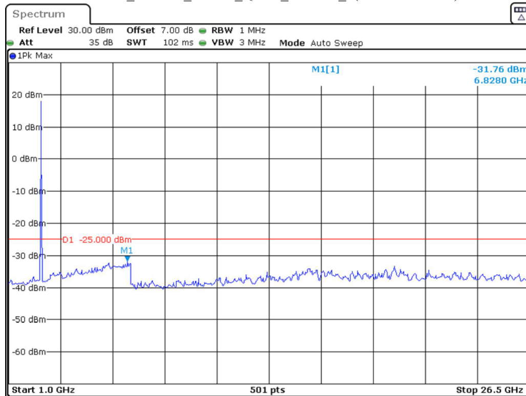
Band 41_15 MHz_Middle_QPSK_RB75#0_2(1GHz-26.5GHz)
