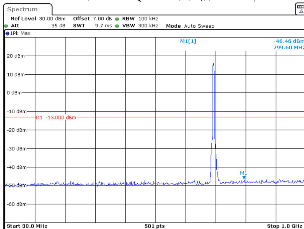
Band 12_5 MHz_Low_QPSK_RB25#0_1(30MHz-1GHz)
