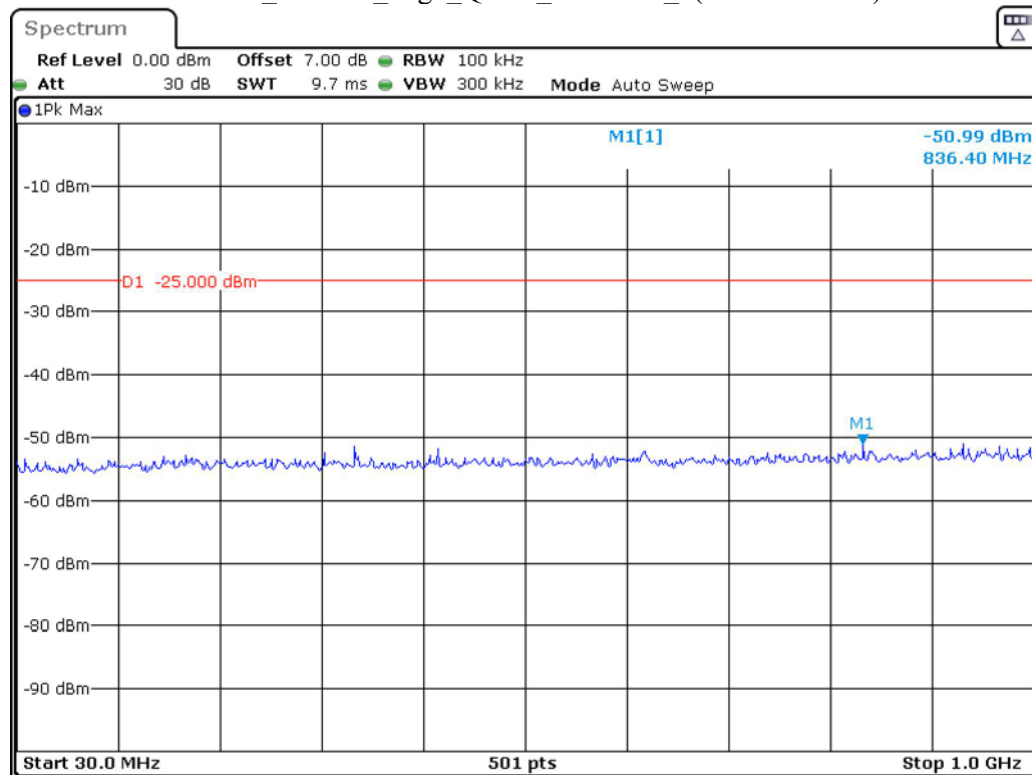
Band 41_20 MHz_High_QPSK_RB100#0_1(30MHz-1GHz)
