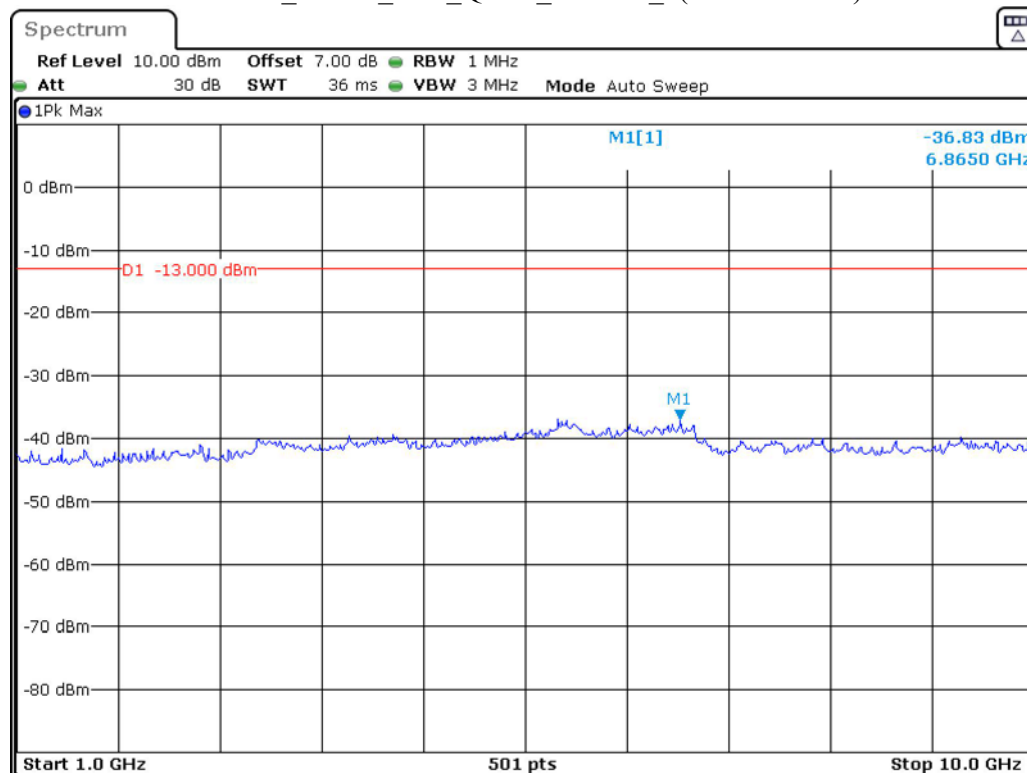
Band 12_5 MHz_Low_QPSK_RB25#0_2(1GHz-10GHz)
