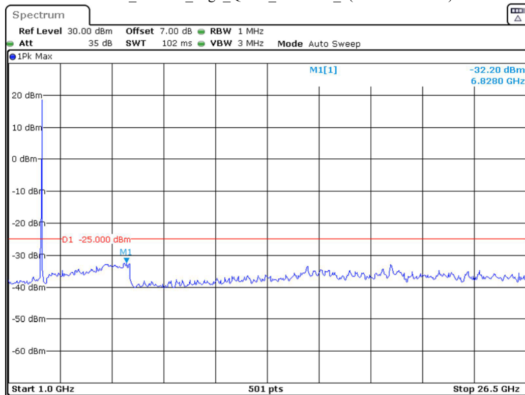
Band 41_20 MHz_High_QPSK_RB100#0_2(1GHz-26.5GHz)
