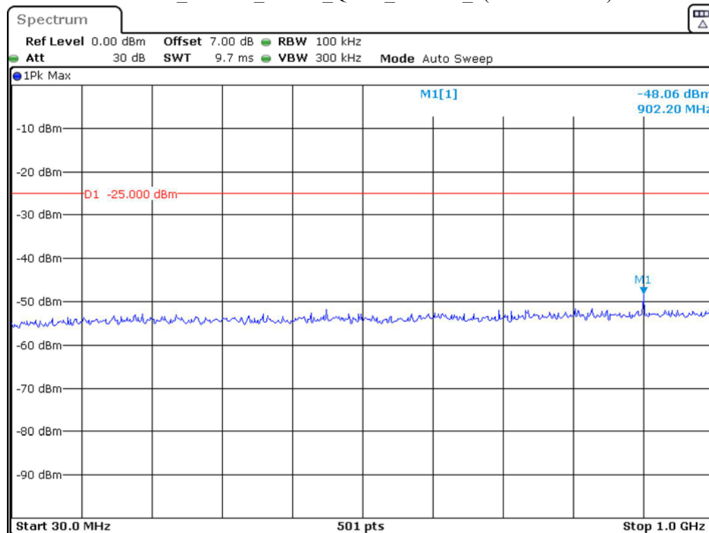
Band 41_15 MHz_Middle_QPSK_RB75#0_1(30MHz-1GHz)
