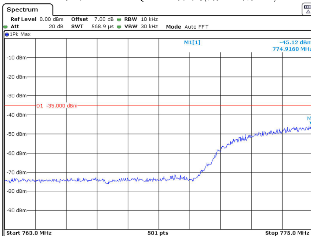
Band 13_10 MHz_Middle_QPSK_RB50#0_3(763MHz-775MHz)
