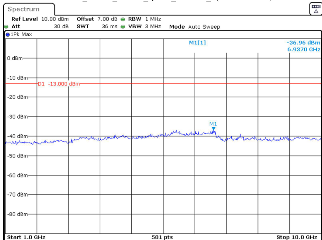
Band 12_5 MHz_Middle_QPSK_RB25#0_2(1GHz-10GHz)
