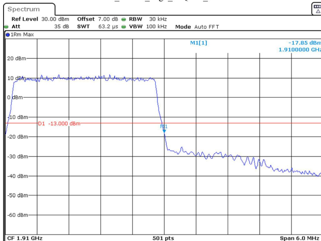
Band 2_3 MHz_High_16QAM_RB15#0
