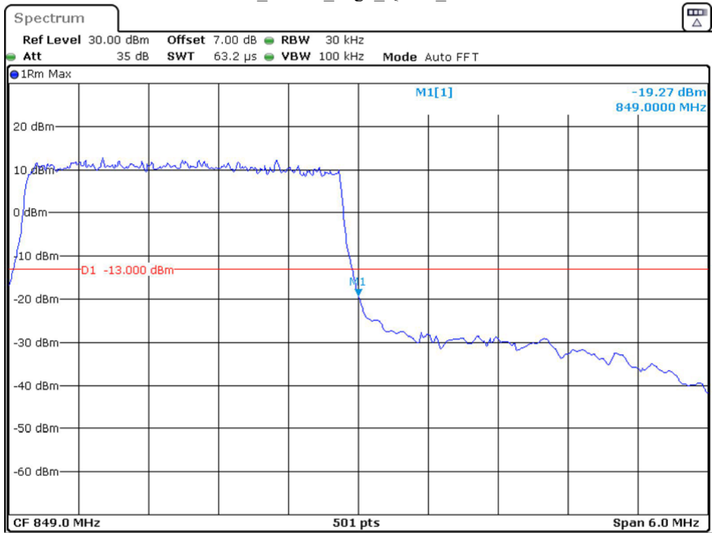
Band 5_3 MHz_High_QPSK_RB15#0
