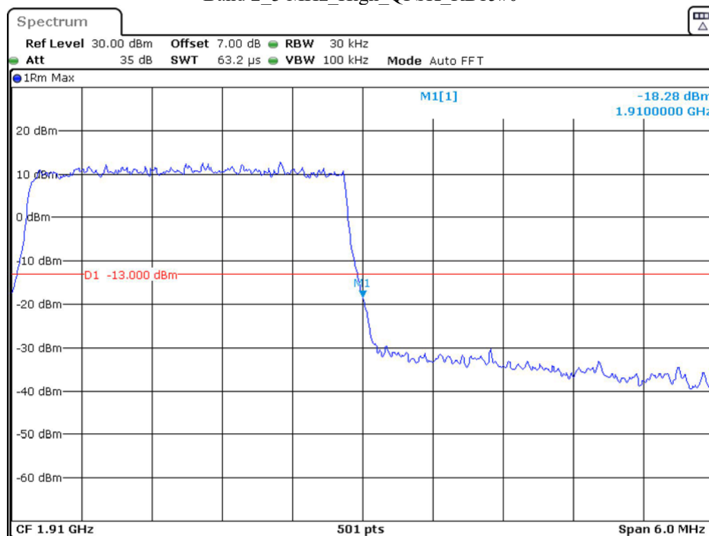
Band 2_3 MHz_High_QPSK_RB15#0
