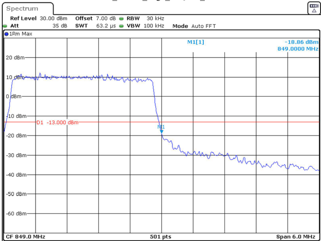
Band 5_3 MHz_High_16QAM_RB15#0
