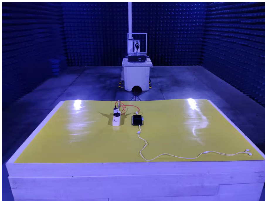
Coaxial View
