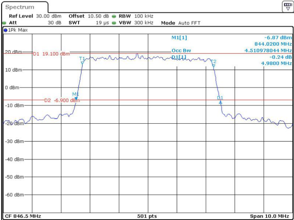
Band 5_5 MHz_High_16QAM_RB25#0
