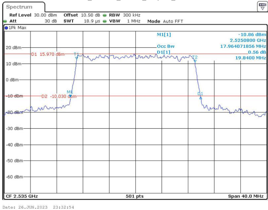
Band 7_20 MHz_Middle_16QAM_RB100#0
