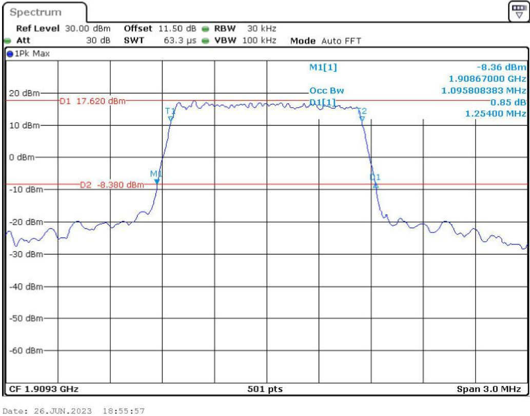
Band 2_1.4 MHz_High_QPSK_RB6#0
