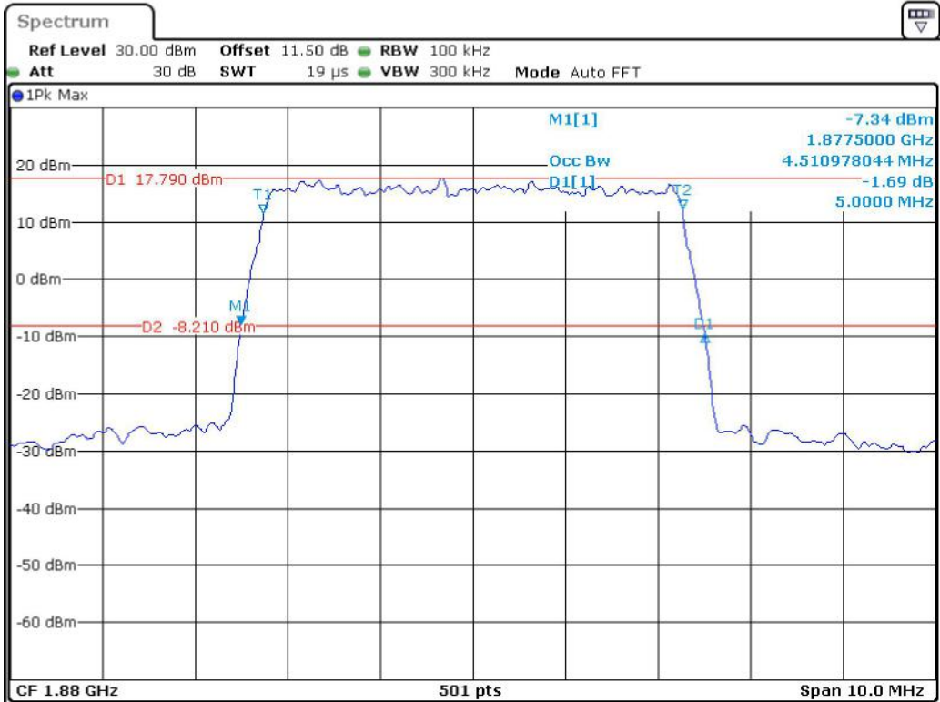
Band 2_5 MHz_Middle_QPSK_RB25#0
