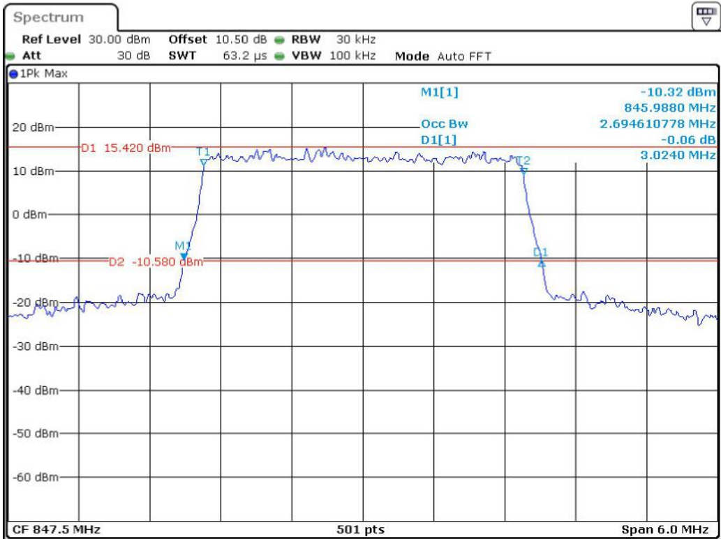
Band 5_3 MHz_High_16QAM_RB15#0
