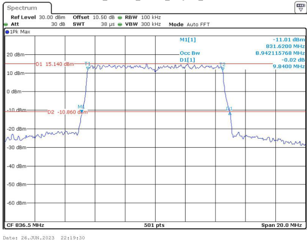
Band 5_10 MHz_Middle_16QAM_RB50#0
