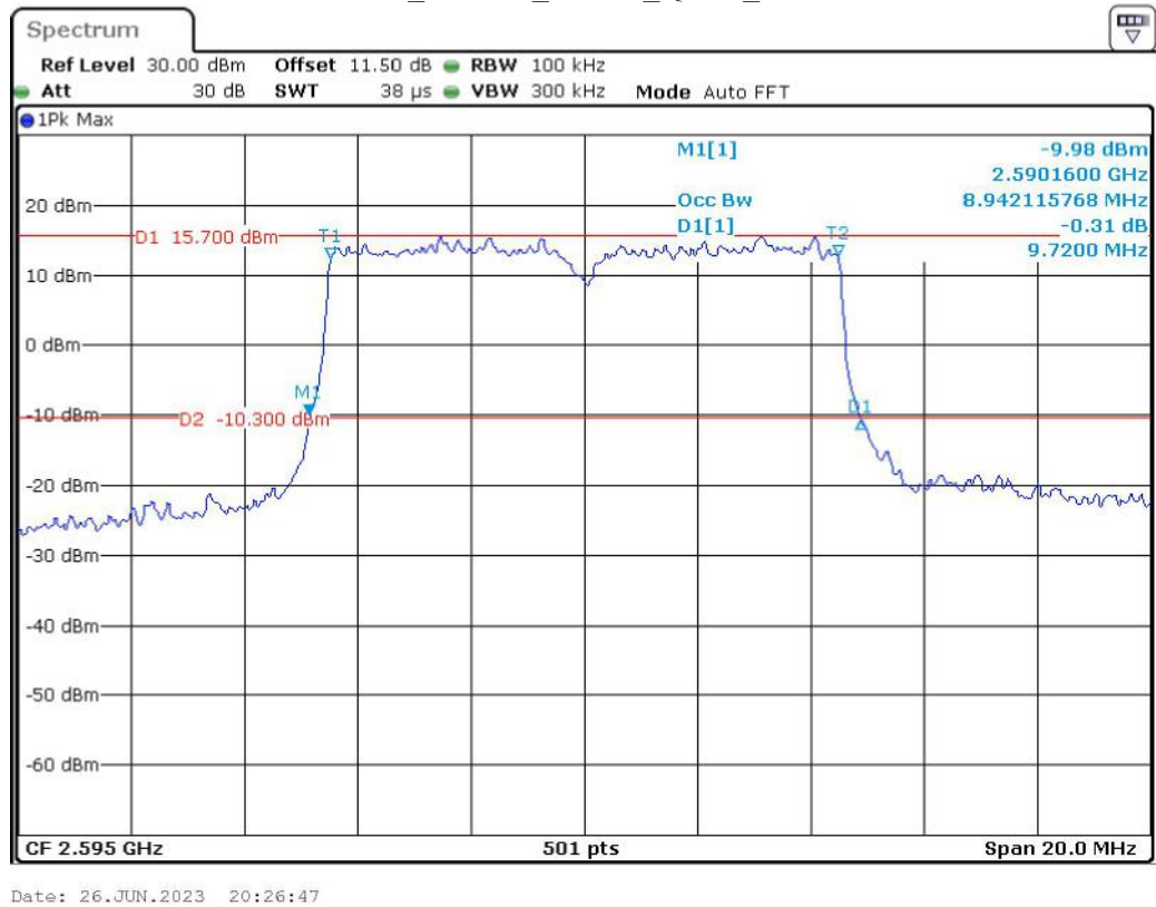
Band 41_10 MHz_Middle_QPSK_RB50#0
