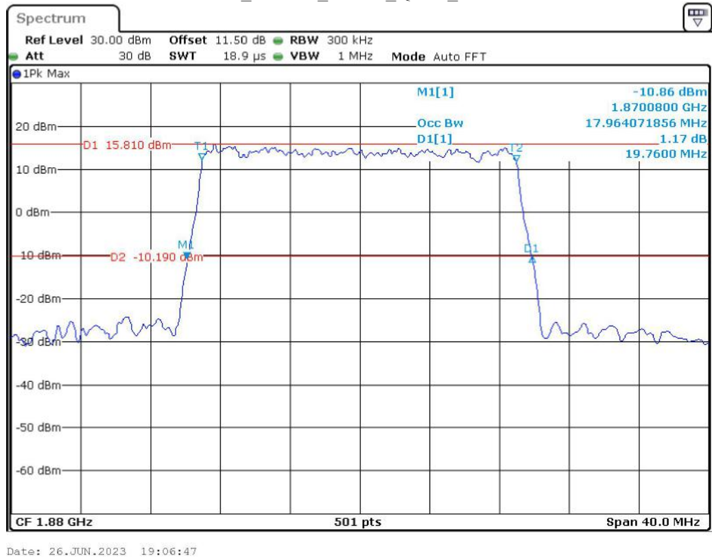
Band 2_20 MHz_Middle_QPSK_RB100#0
