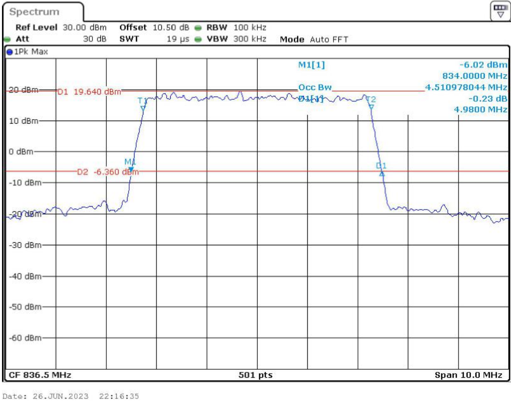
Band 5_5 MHz_Middle_QPSK_RB25#0
