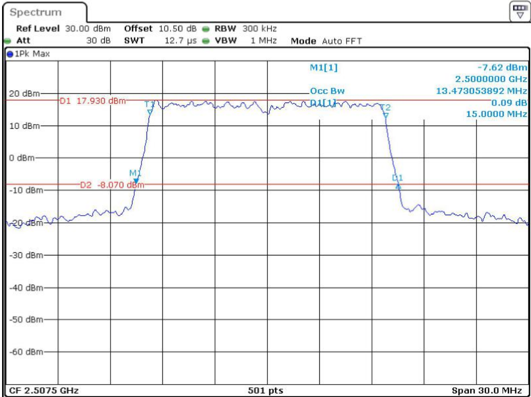
Band 7_15 MHz_Low_QPSK_RB75#0
