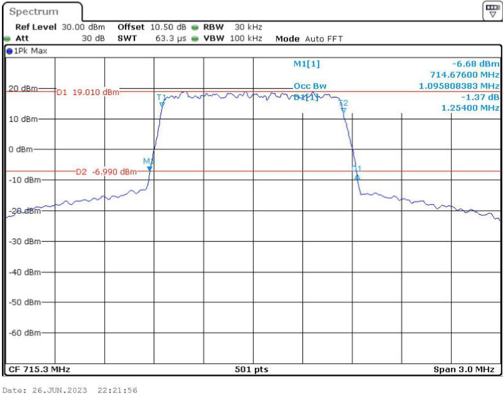
Band 12_1.4 MHz_High_QPSK_RB6#0
