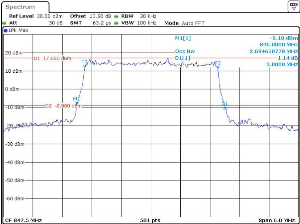
Band 5_3 MHz_High_QPSK_RB15#0
