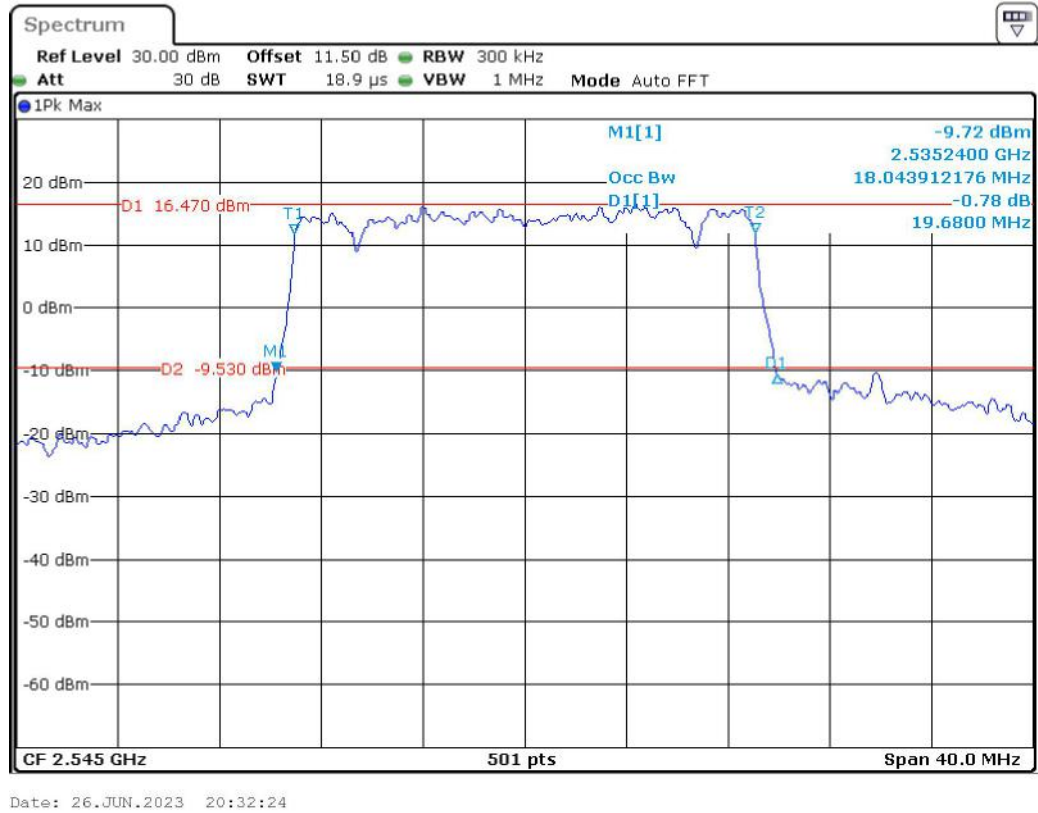
Band 41_20 MHz_Low_16QAM_RB100#0
