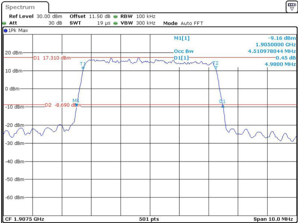
Band 2_5 MHz_High_16QAM_RB25#0
