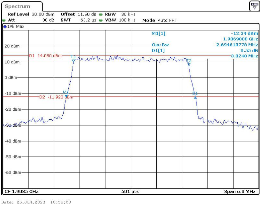
Band 2_3 MHz_High_16QAM_RB15#0
