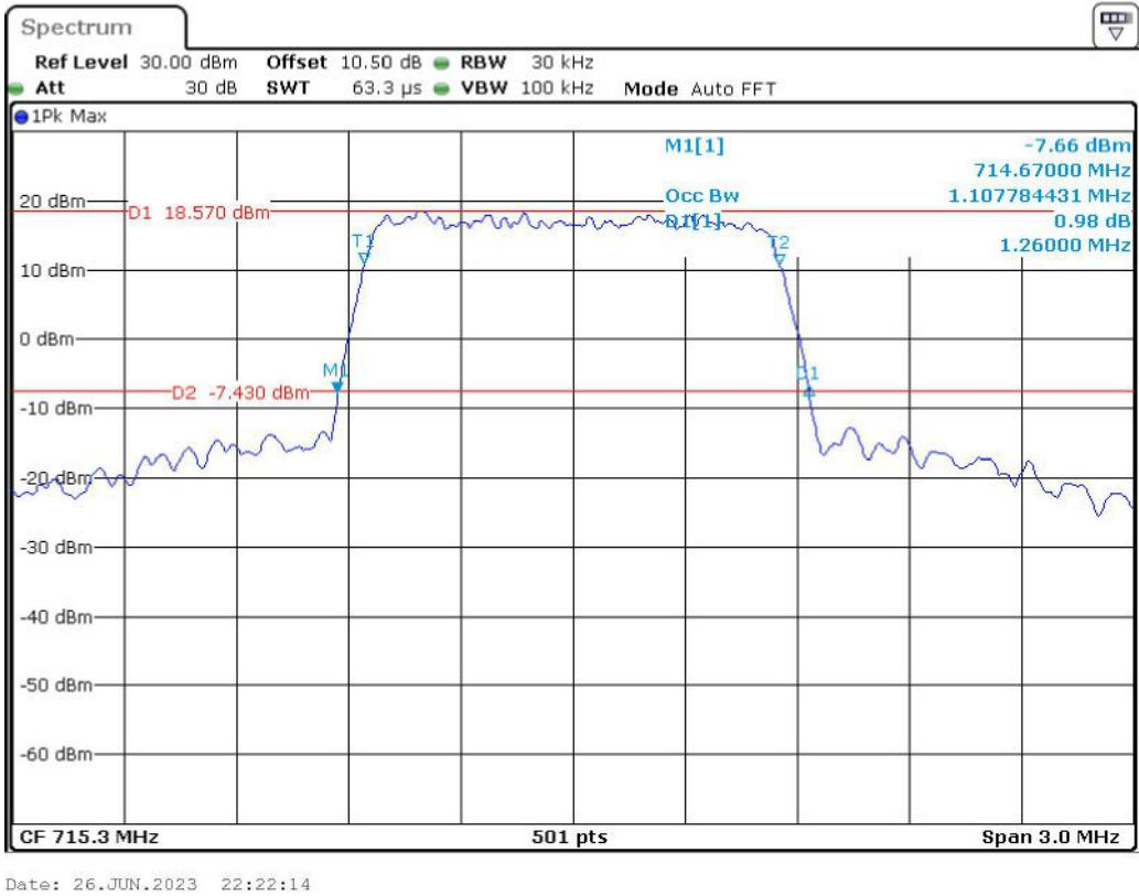
Band 12_1.4 MHz_High_16QAM_RB6#0
