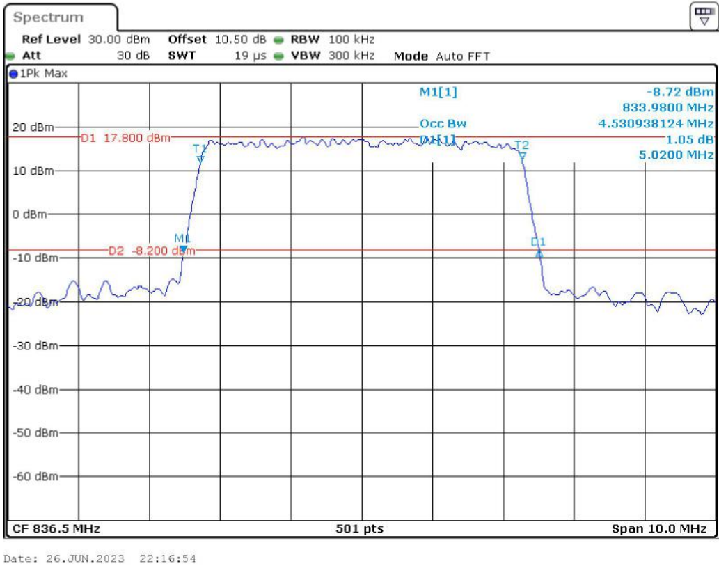
Band 5_5 MHz_Middle_16QAM_RB25#0
