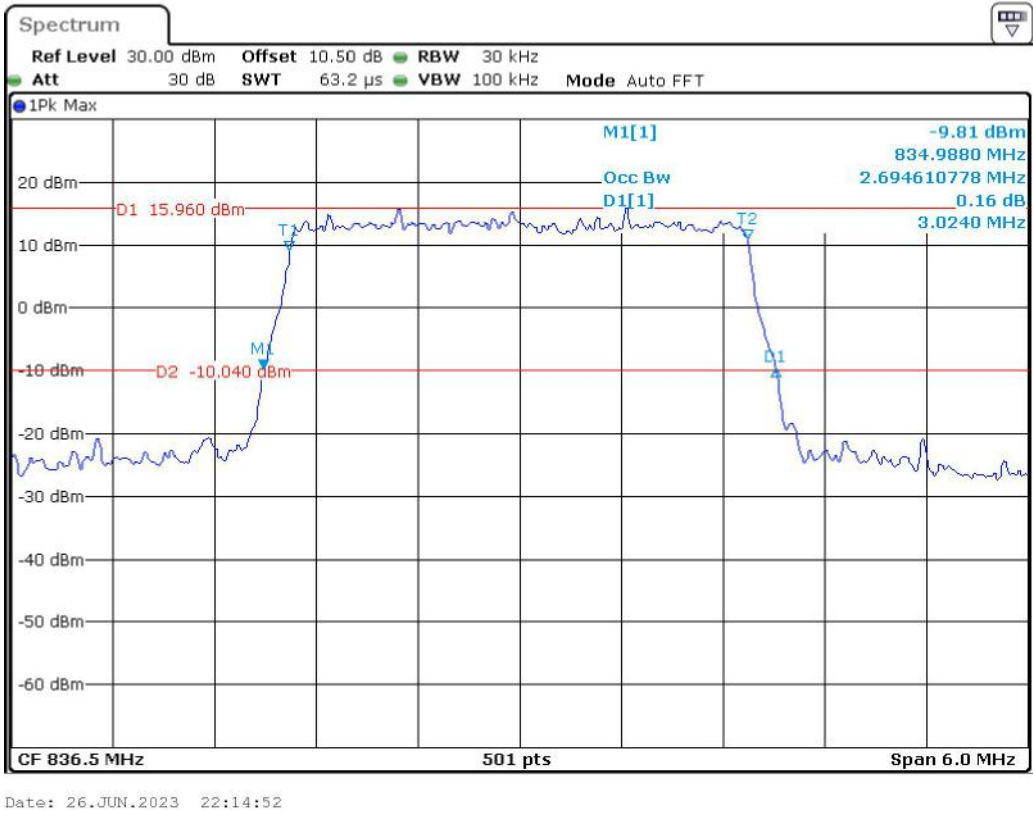
Band 5_3 MHz_Middle_16QAM_RB15#0
