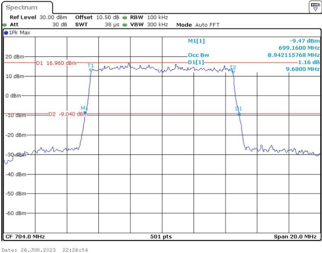
Band 12_10 MHz_Low_QPSK_RB50#0
