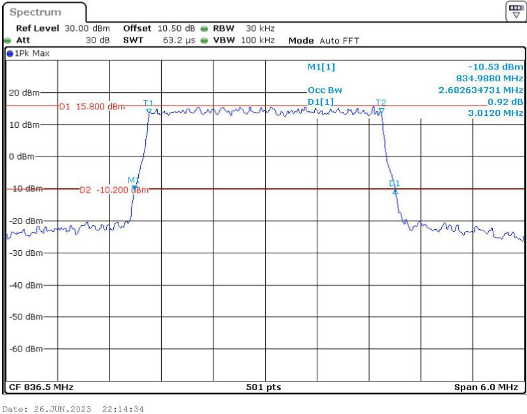
Band 5_3 MHz_Middle_QPSK_RB15#0
