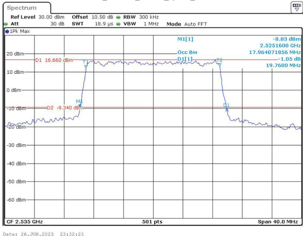
Band 7_20 MHz_Middle_QPSK_RB100#0
