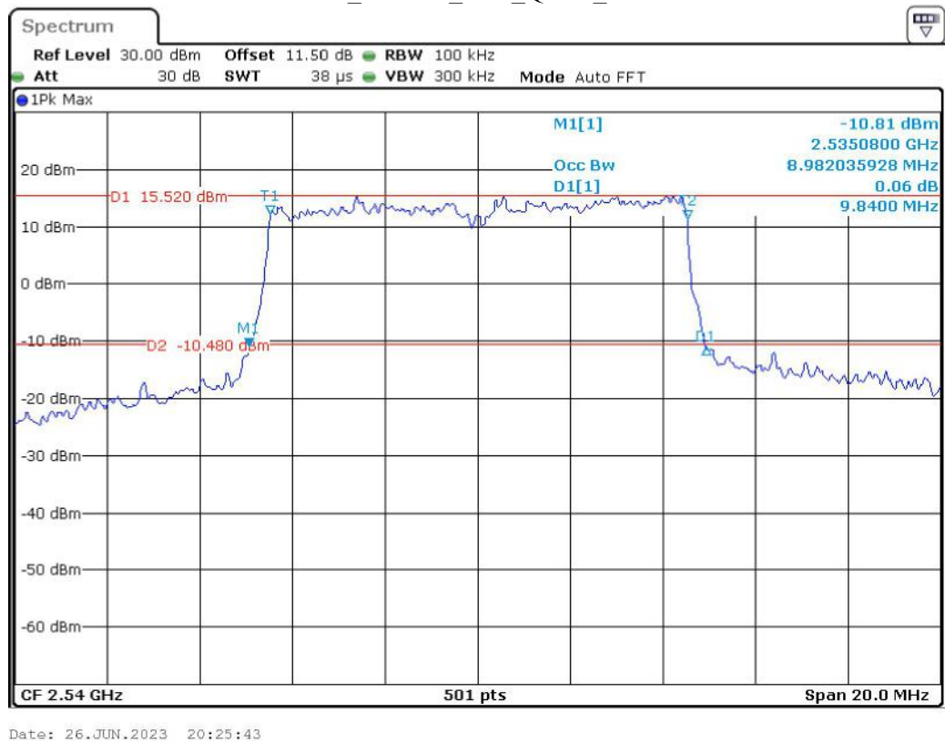
Band 41_10 MHz_Low_QPSK_RB50#0
