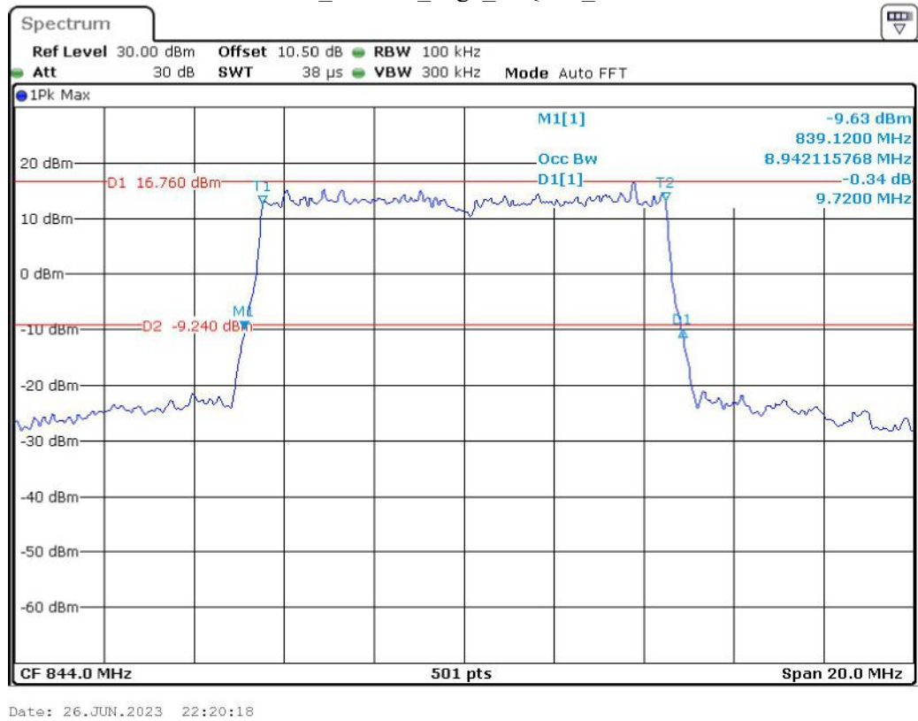
Band 5_10 MHz_High_16QAM_RB50#0
