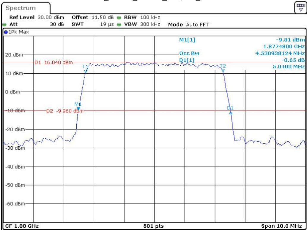
Band 2_5 MHz_Middle_16QAM_RB25#0
