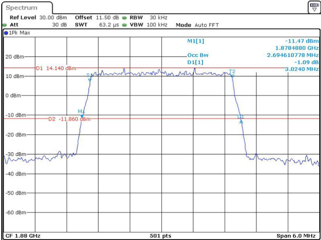
Band 2_3 MHz_Middle_16QAM_RB15#0
