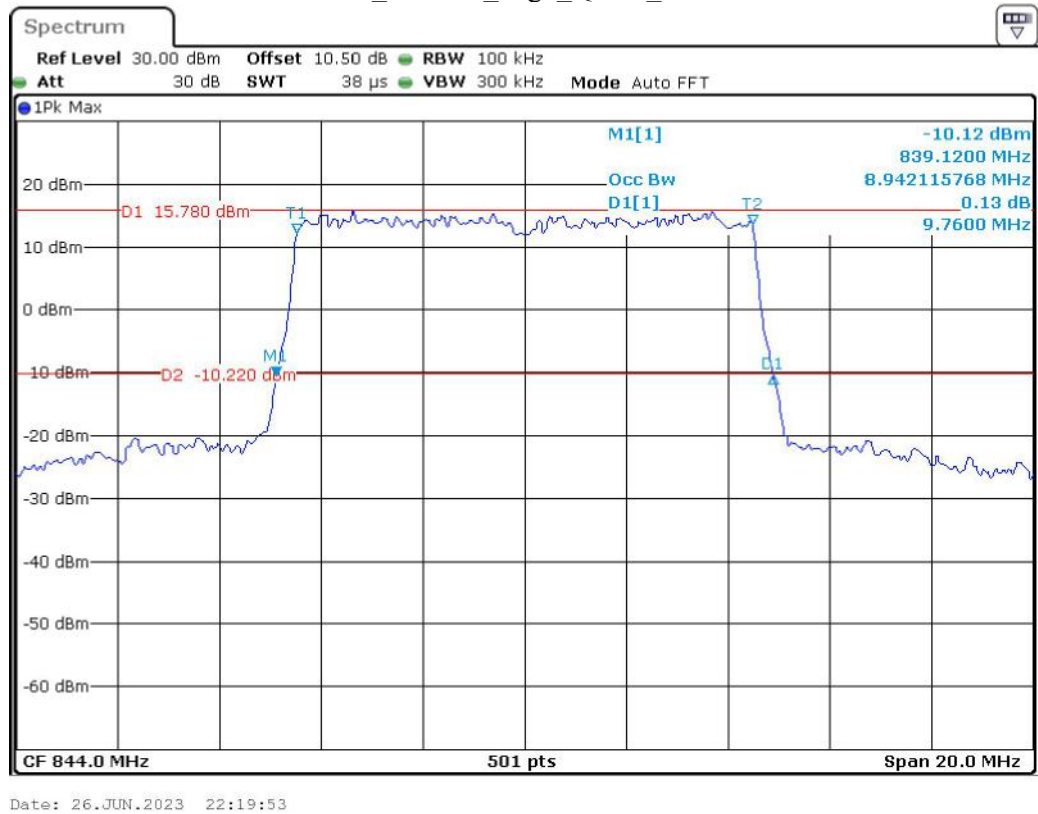
Band 5_10 MHz_High_QPSK_RB50#0
