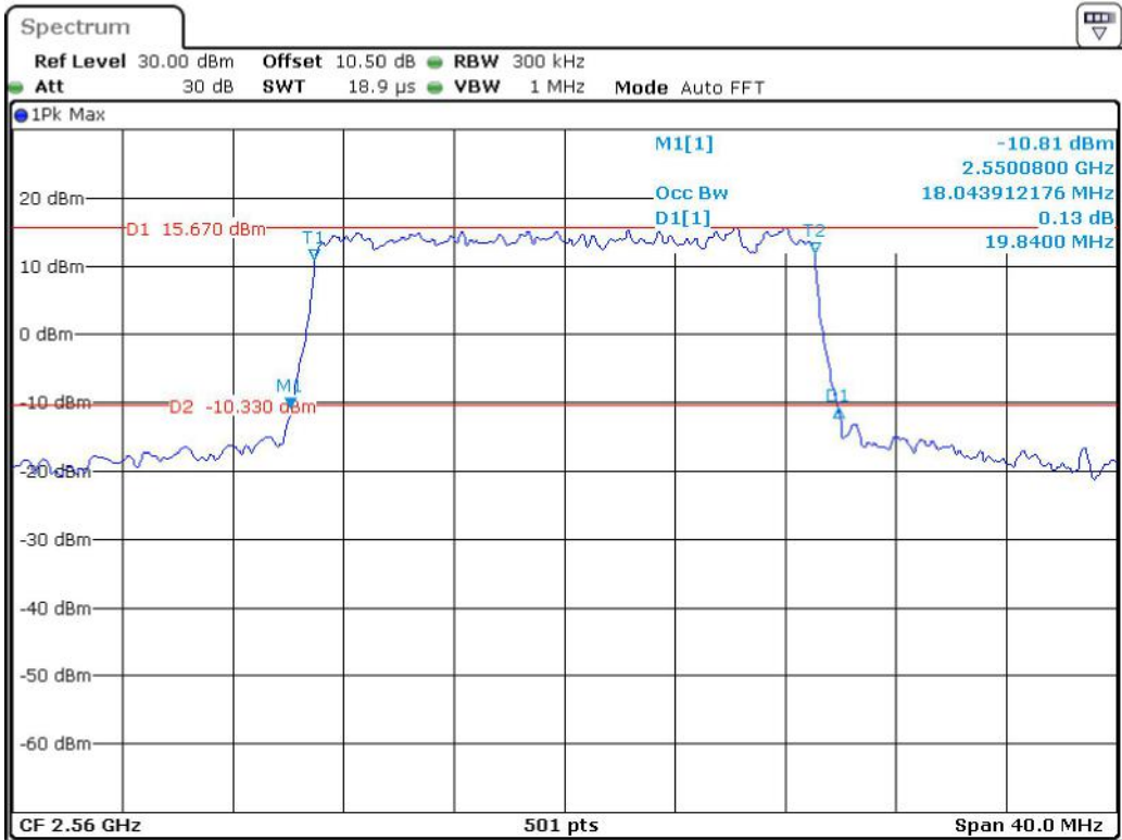
Band 7_20 MHz_High_16QAM_RB100#0
