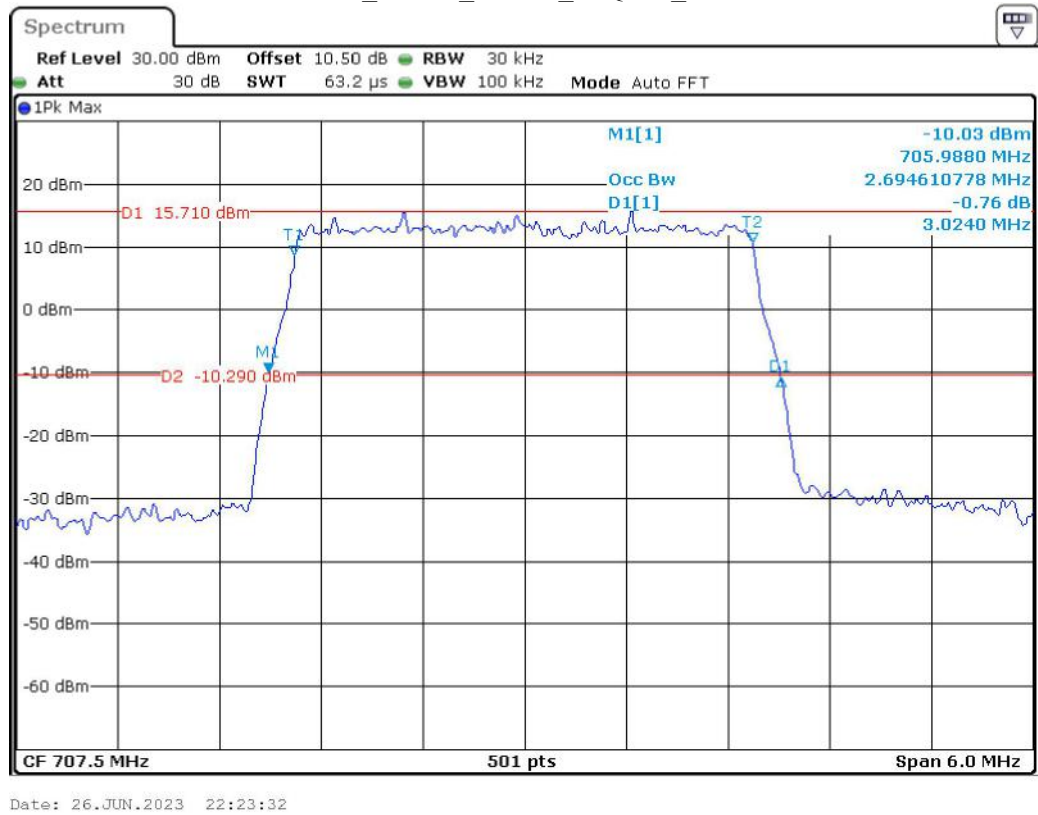
Band 12_3 MHz_Middle_16QAM_RB15#0
