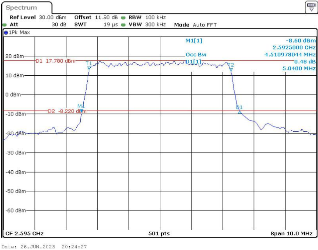
Band 41_5 MHz_Middle_16QAM_RB25#0
