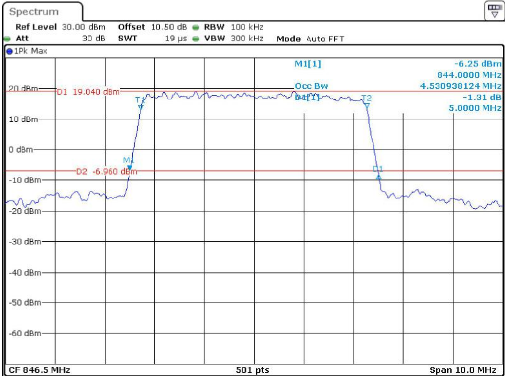
Band 5_5 MHz_High_QPSK_RB25#0
