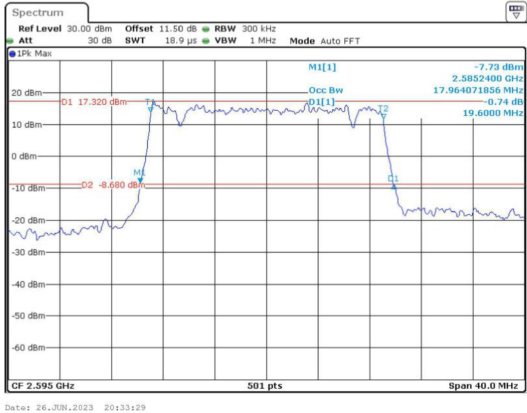
Band 41_20 MHz_Middle_16QAM_RB100#0
