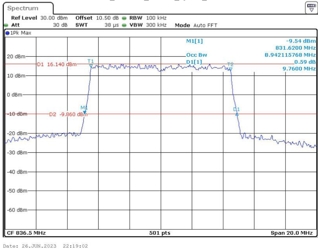
Band 5_10 MHz_Middle_QPSK_RB50#0
