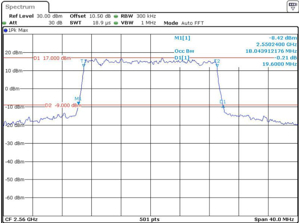
Band 7_20 MHz_High_QPSK_RB100#0
