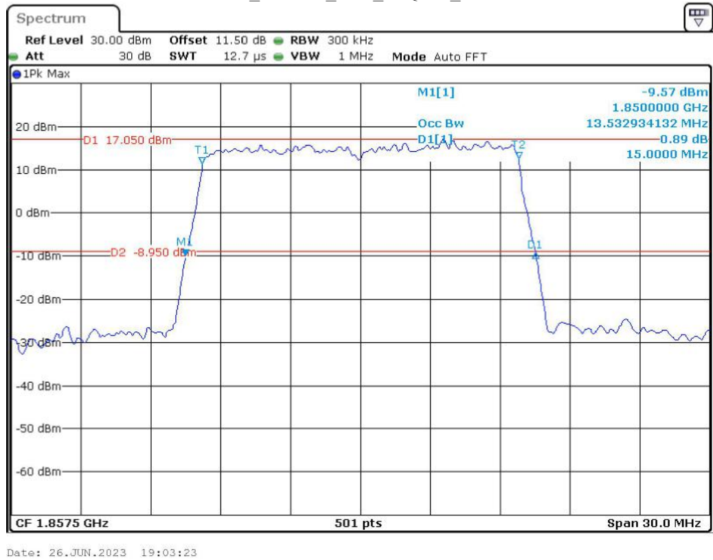
Band 2_15 MHz_Low_16QAM_RB75#0
