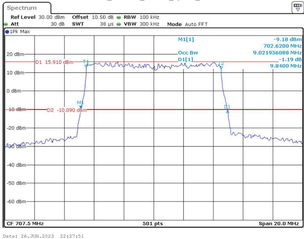
Band 12_10 MHz_Middle_QPSK_RB50#0
