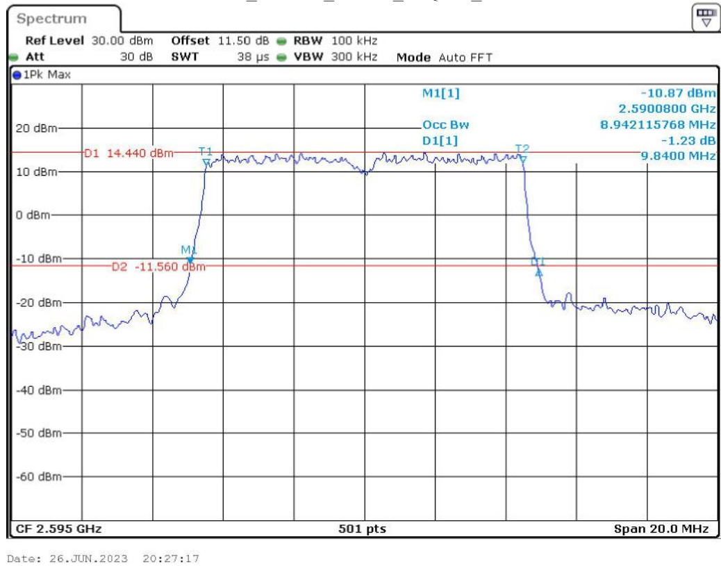
Band 41_10 MHz_Middle_16QAM_RB50#0
