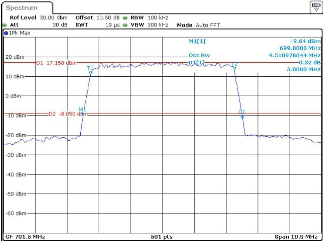
Band 12_5 MHz_Low_16QAM_RB25#0
