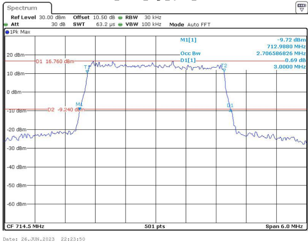
Band 12_3 MHz_High_QPSK_RB15#0
