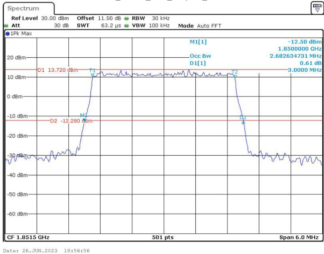
Band 2_3 MHz_Low_16QAM_RB15#0
