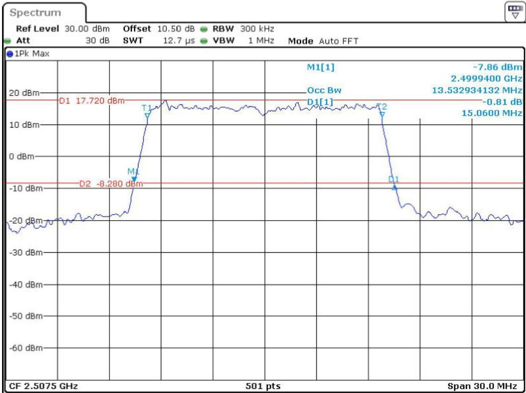
Band 7_15 MHz_Low_16QAM_RB75#0
