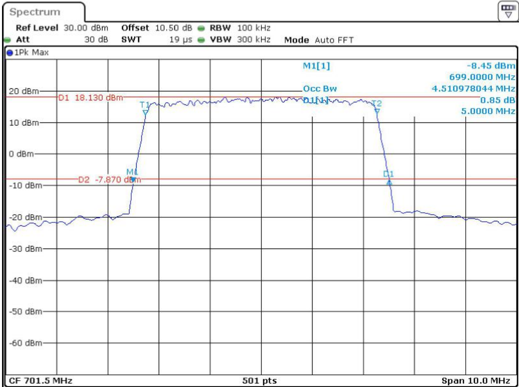
Band 12_5 MHz_Low_QPSK_RB25#0
