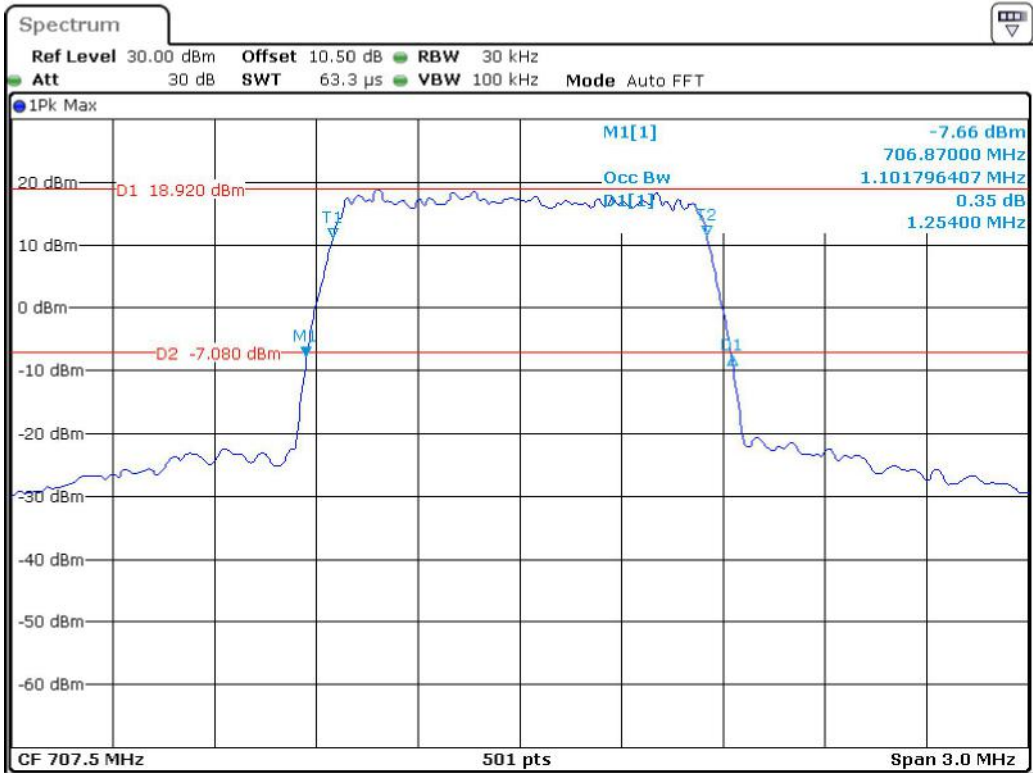
Band 12_1.4 MHz_Middle_16QAM_RB6#0
