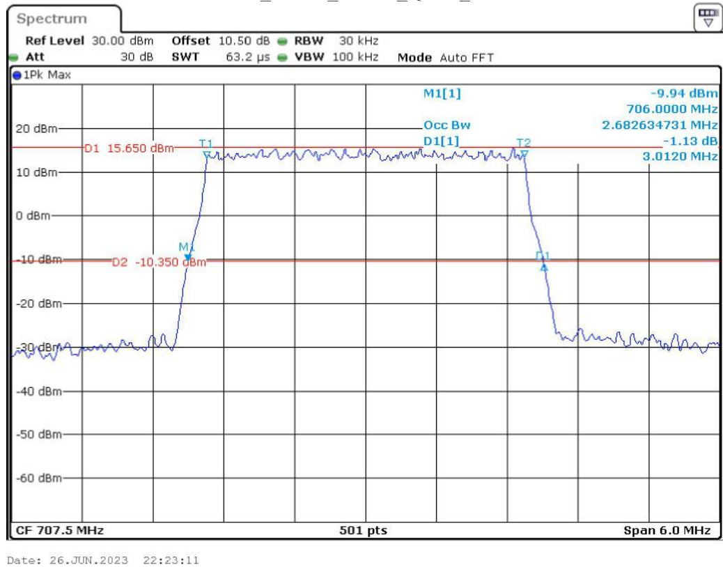
Band 12_3 MHz_Middle_QPSK_RB15#0
