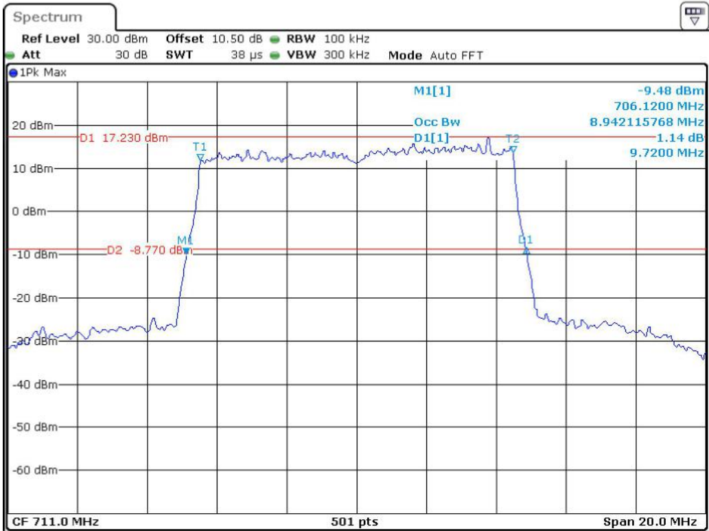
Band 12_10 MHz_High_16QAM_RB50#0
