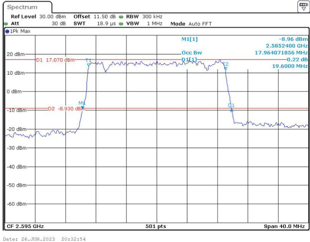
Band 41_20 MHz_Middle_QPSK_RB100#0
