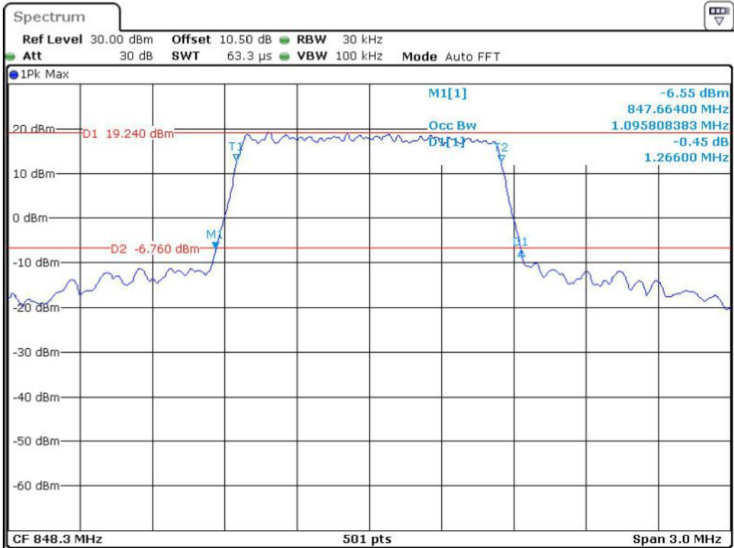
Band 5_1.4 MHz_High_QPSK_RB6#0
