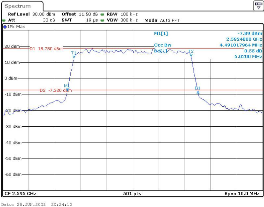
Band 41_5 MHz_Middle_QPSK_RB25#0
