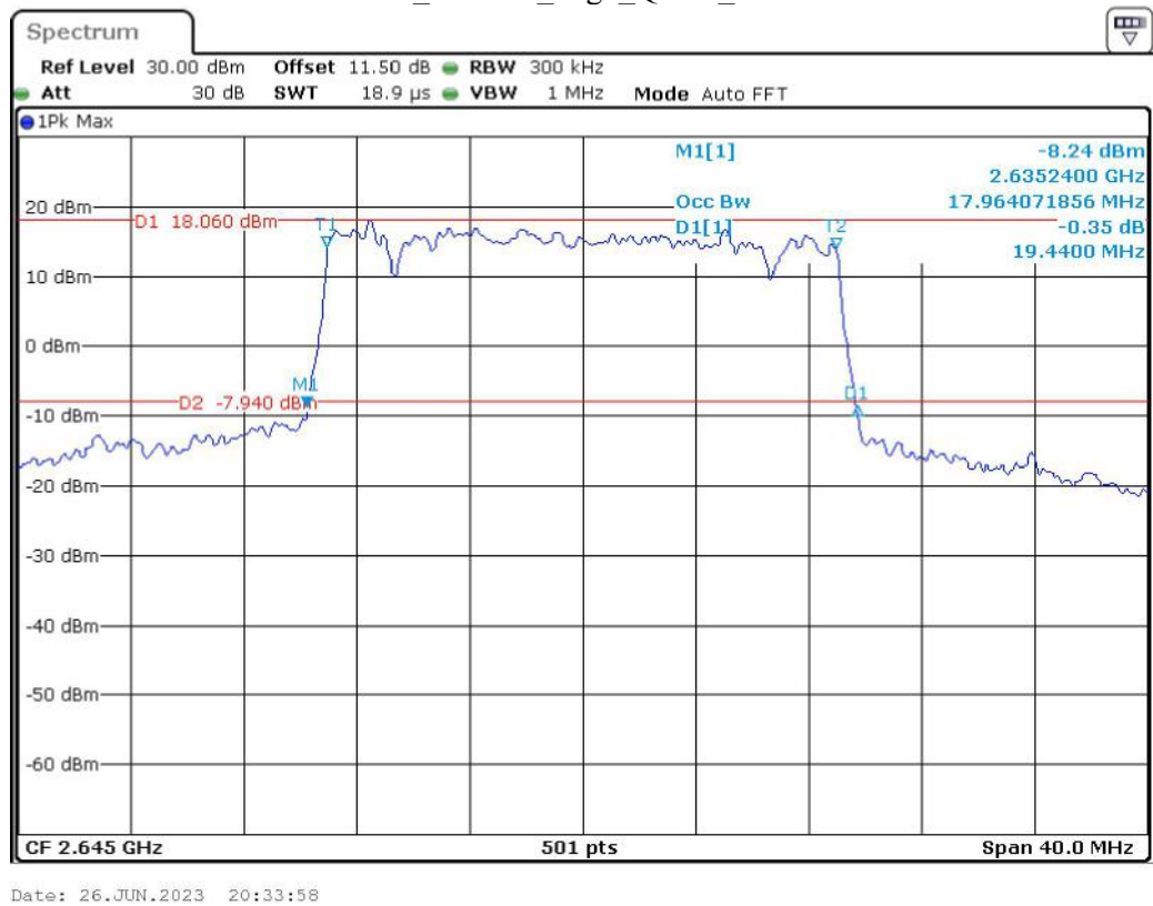
Band 41_20 MHz_High_QPSK_RB100#0
