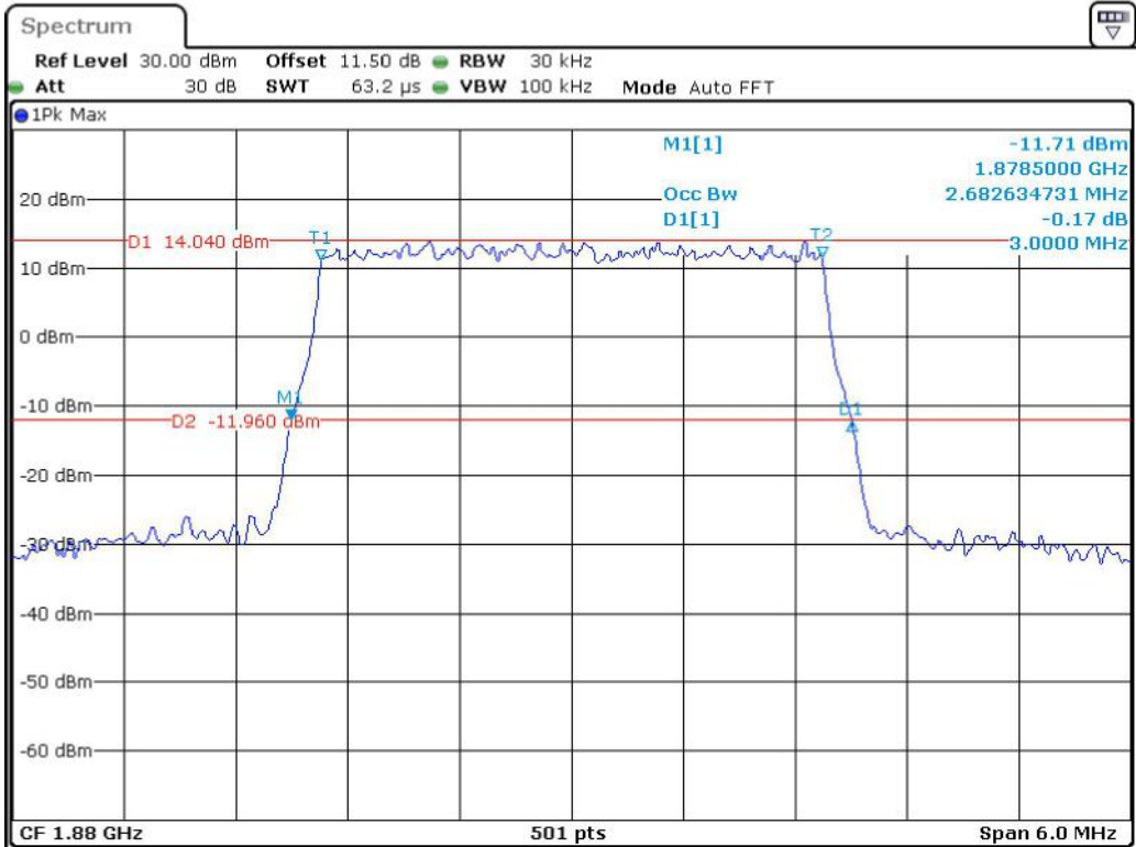
Band 2_3 MHz_Middle_QPSK_RB15#0
