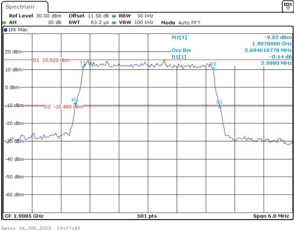
Band 2_3 MHz_High_QPSK_RB15#0
