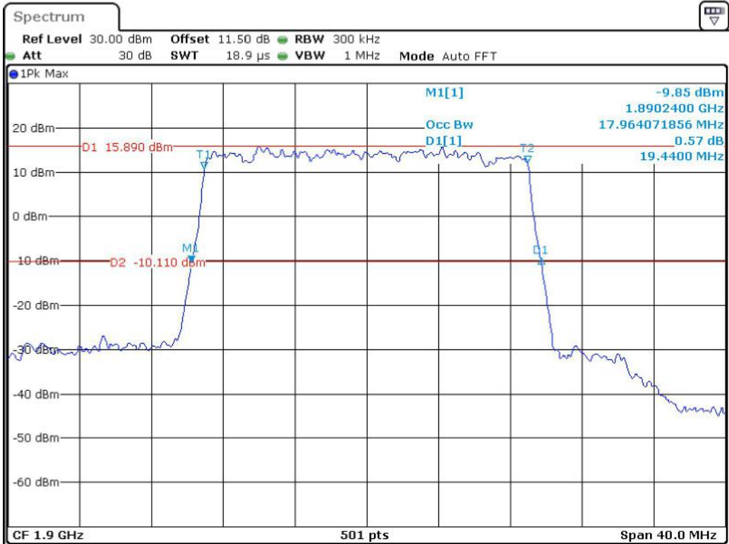
Band 2_20 MHz_High_QPSK_RB100#0
