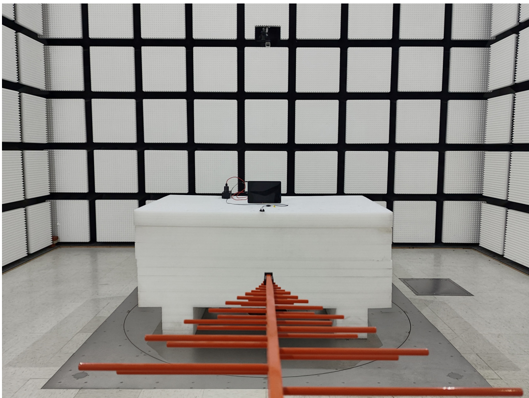
Radiated Emission Below 1G View (HJ-0502000W2-US)
