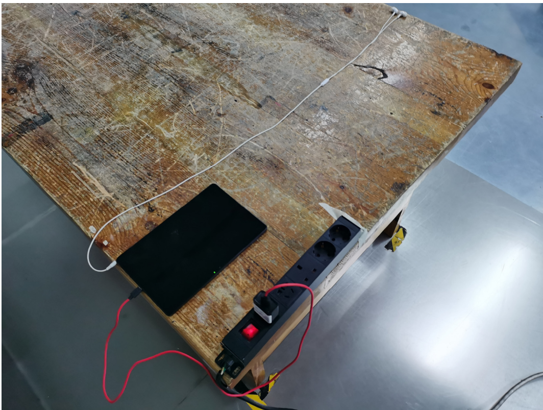
Conducted Emissions Side View (HF-0502000U)
