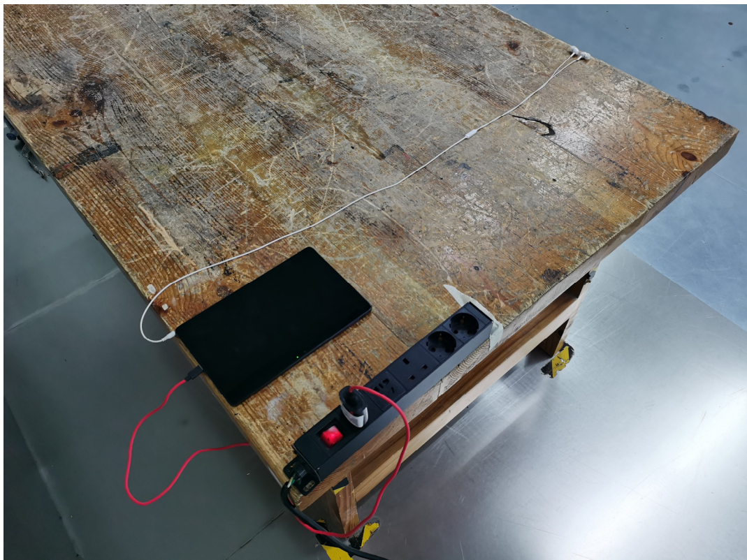
Conducted Emissions Side View (HJ-0502000W2-US)
