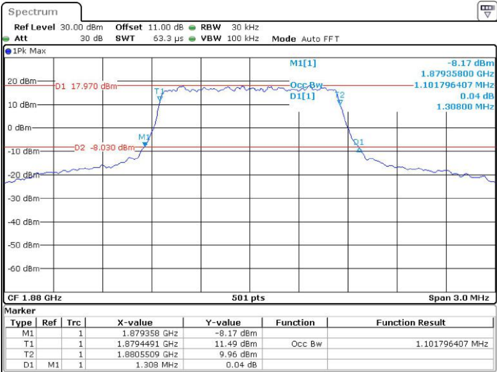
Band 2_1.4 MHz_Middle_QPSK_RB6#0
