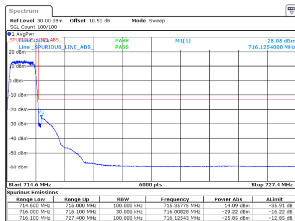
1.4MHz_High_QPSK_6@0
