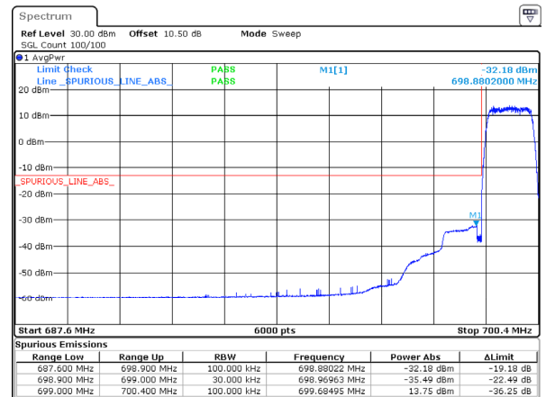
1.4MHz_Low_QPSK_6@0
