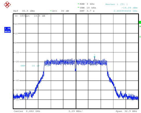
802.11g_2462MHz
