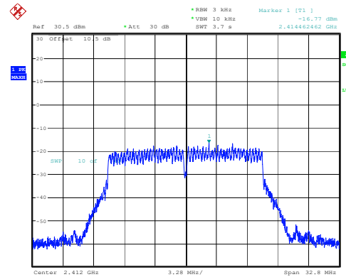
802.11g_2412MHz
