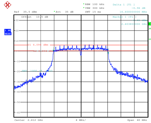
802.11g_2412MHz
