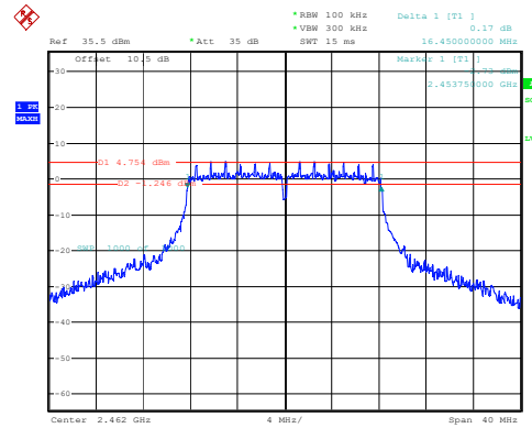
802.11g_2462MHz
