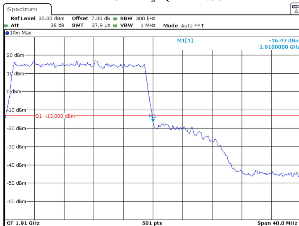
Band 2_20 MHz_High_QPSK_RB100#0
