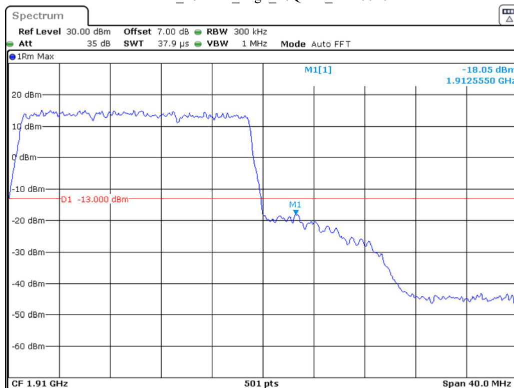
Band 2_20 MHz_High_16QAM_RB100#0
