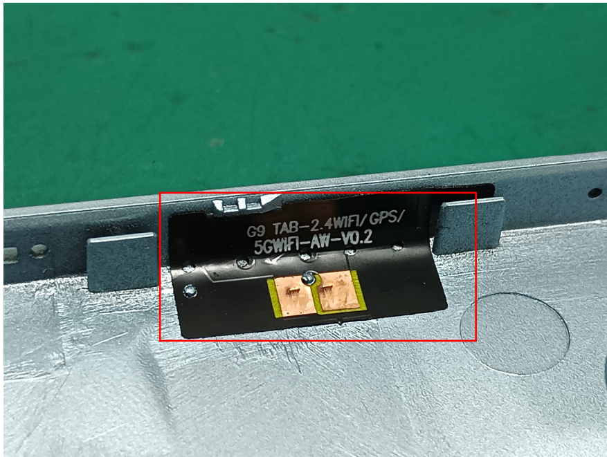
BT/Wi-Fi ANT
