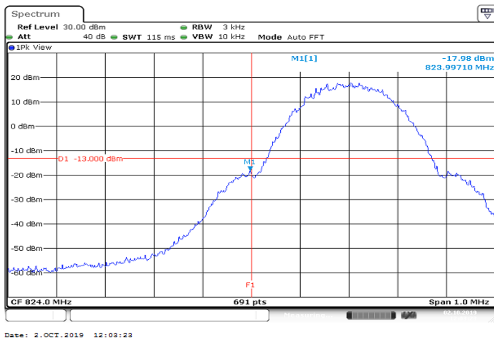
Figure 10-1: Band Edge emissions – GPRS CH Low
