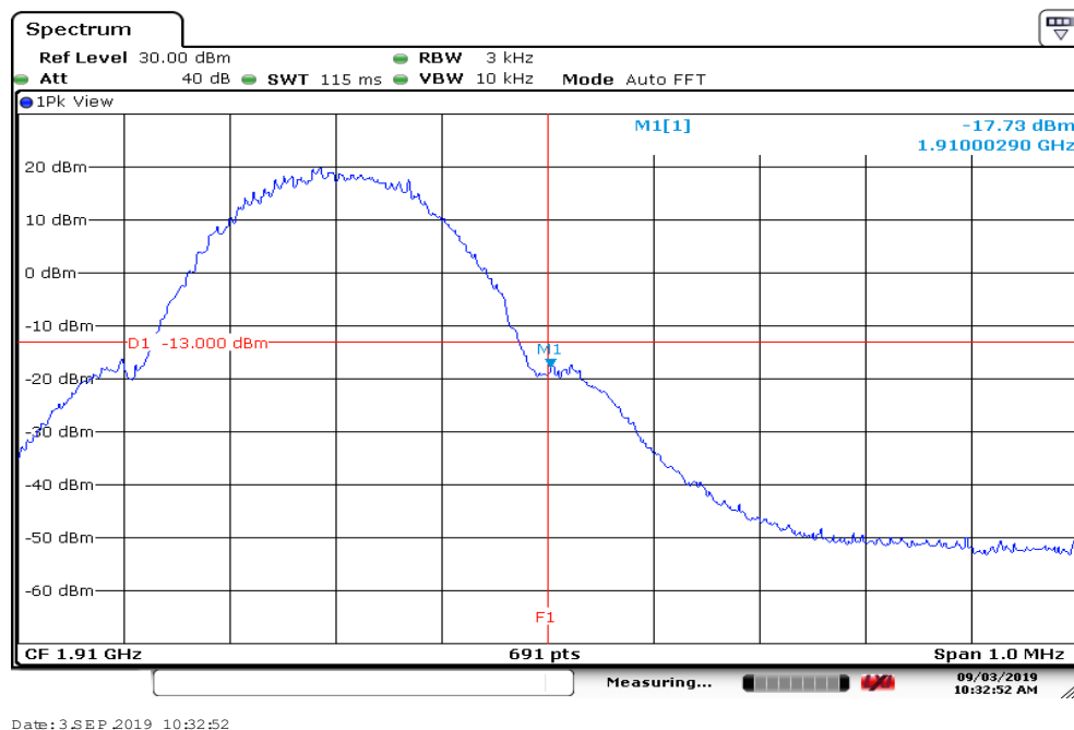
Figure 11-2: Band Edge emissions – GPRS CH High
