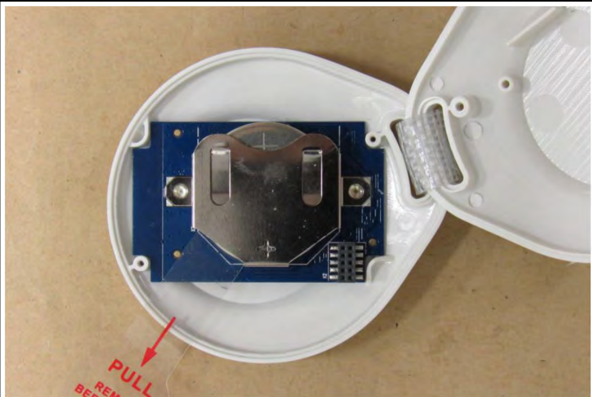
Transponder PCB top (Not tested variant)
