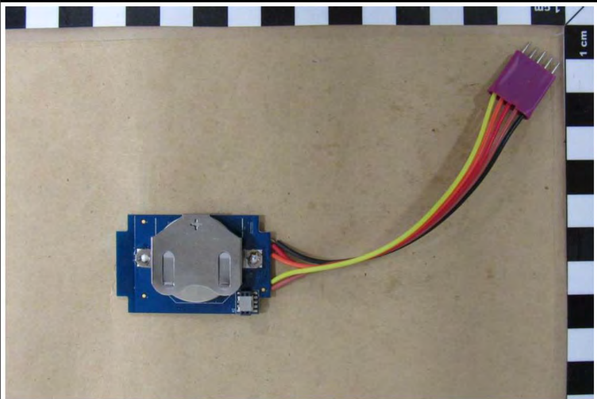
Tested EUT - NosoEx Sensormodul PCB top
