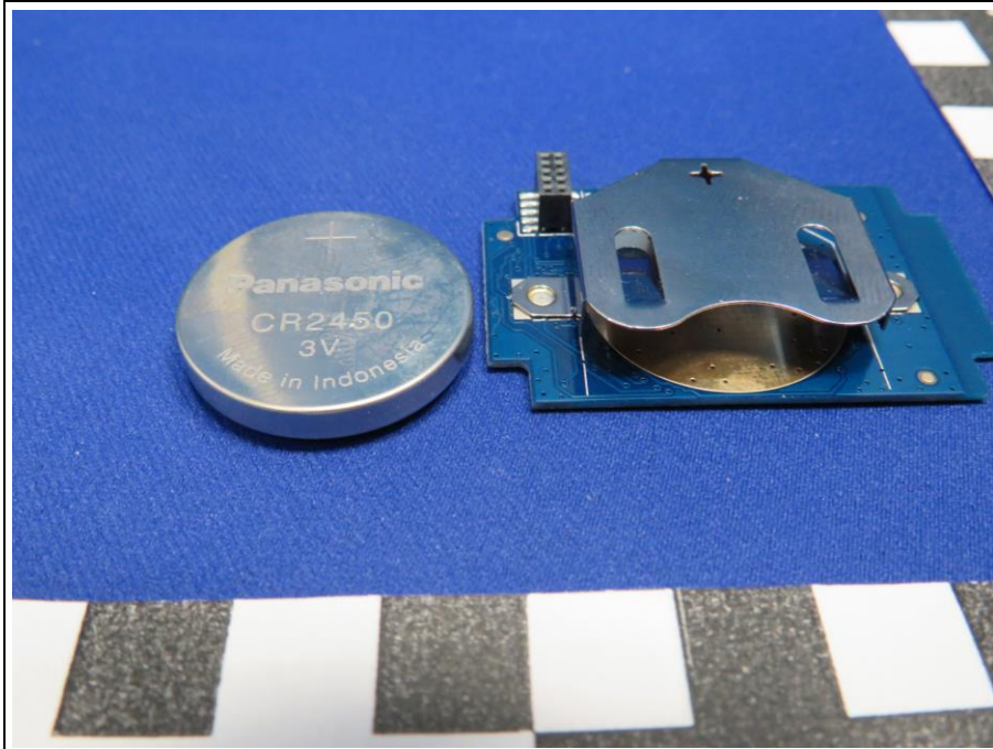
PCB with internal battery
