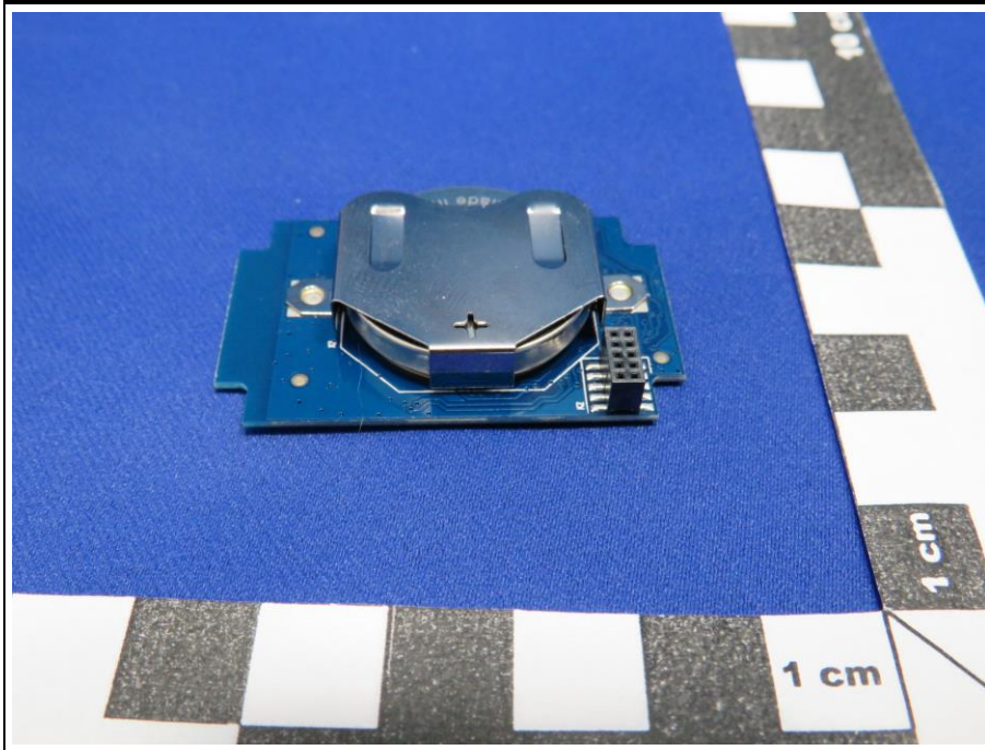
PCB_lower
