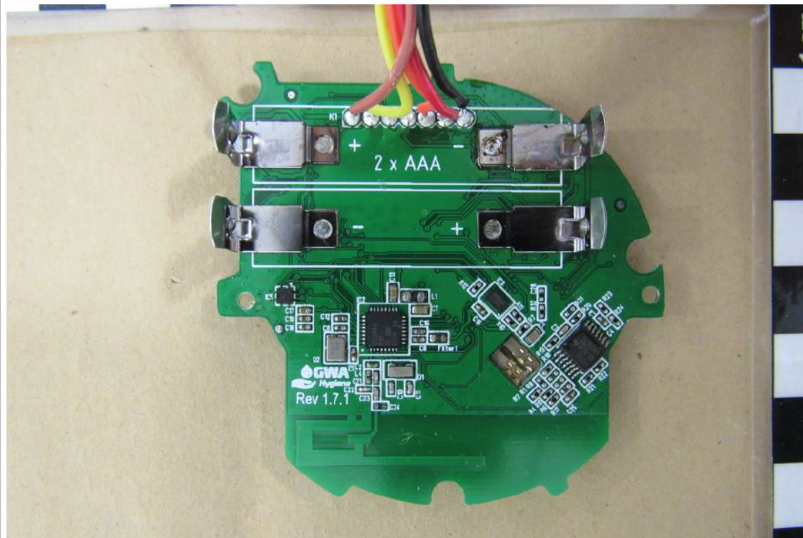
EUT PCB bottom view
