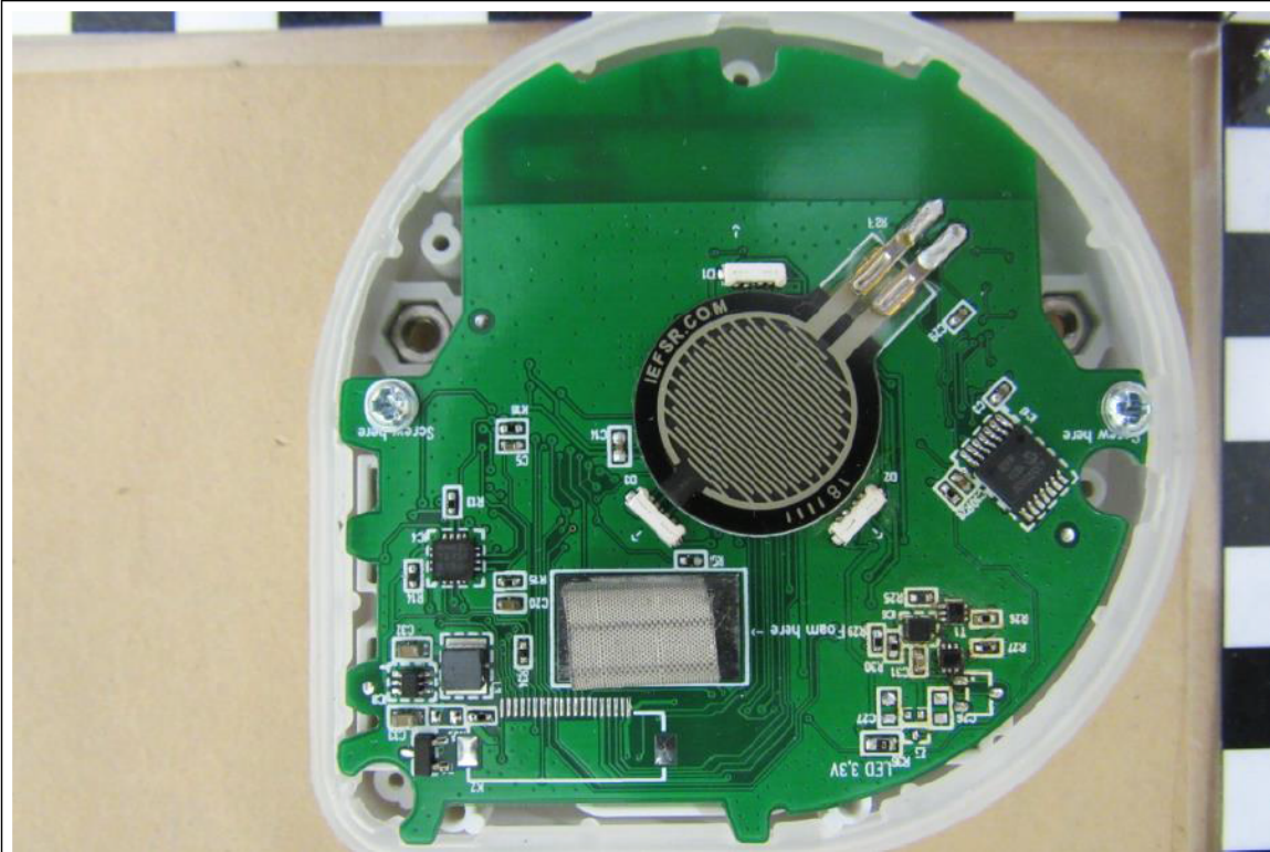
EUT PCB top view
