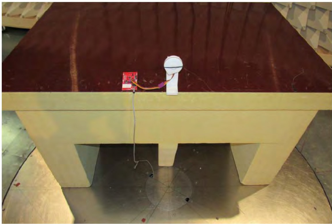
Test Setup close view below 1 GHz
