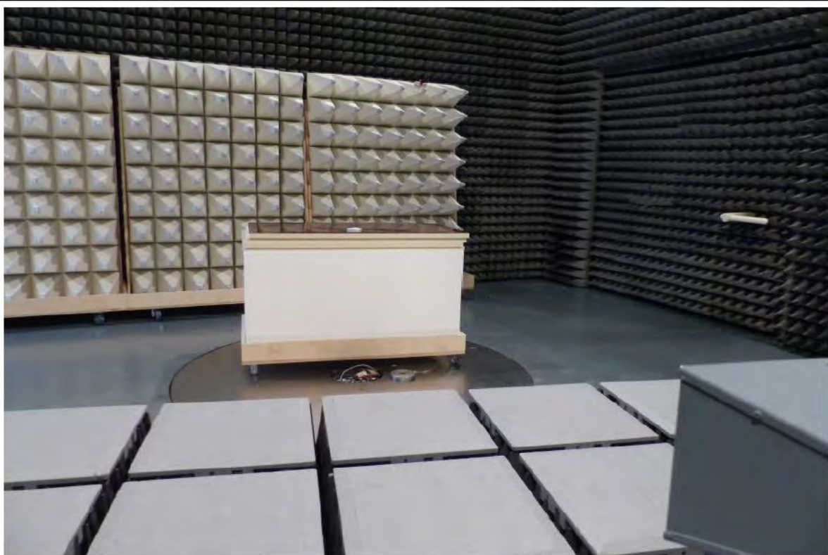
Test setup 1-13GHz
