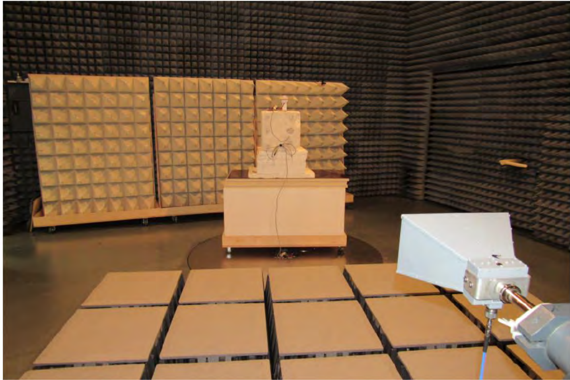
Test Setup 1 - 17 GHz
