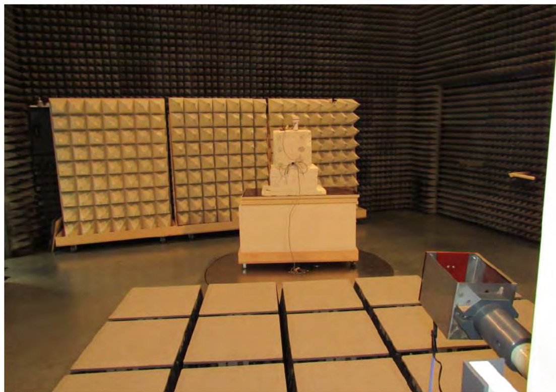
Test Setup 17 - 26 GHz
