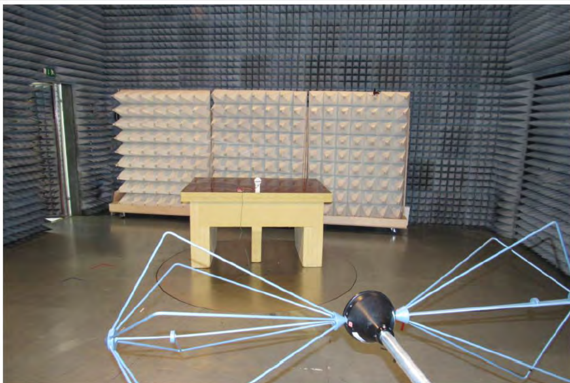
Test Setup 30 - 200 MHz
