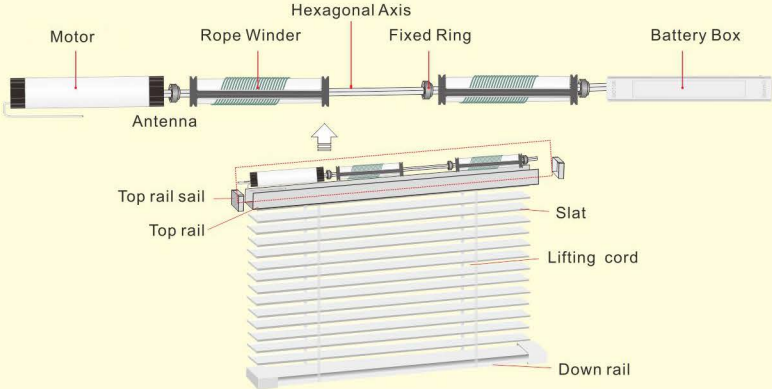
Diagram of the venetian blinds
