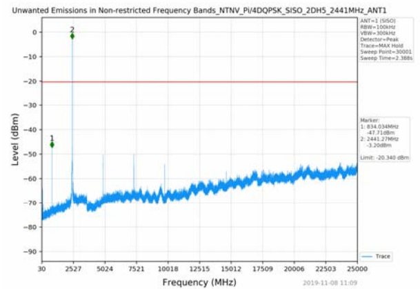
CH39 30MHz-25GHz
