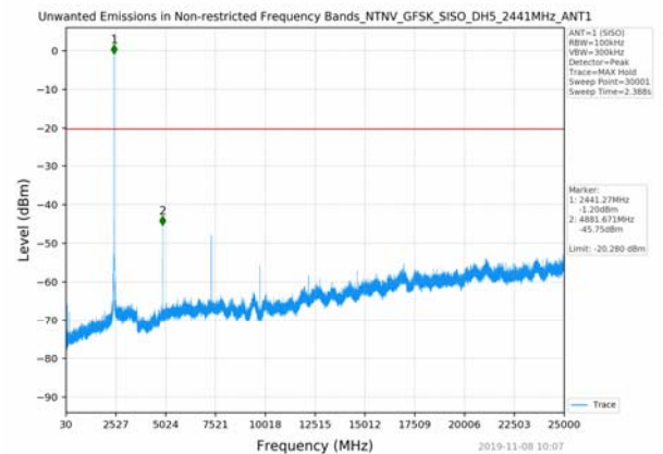
CH39 30MHz-25GHz
