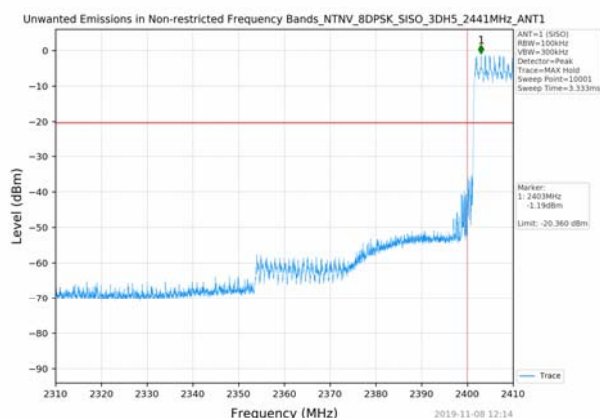
Left Band edge hopping on
