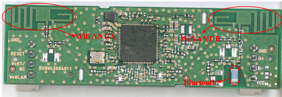
Figure 3 Inside of the EUT
