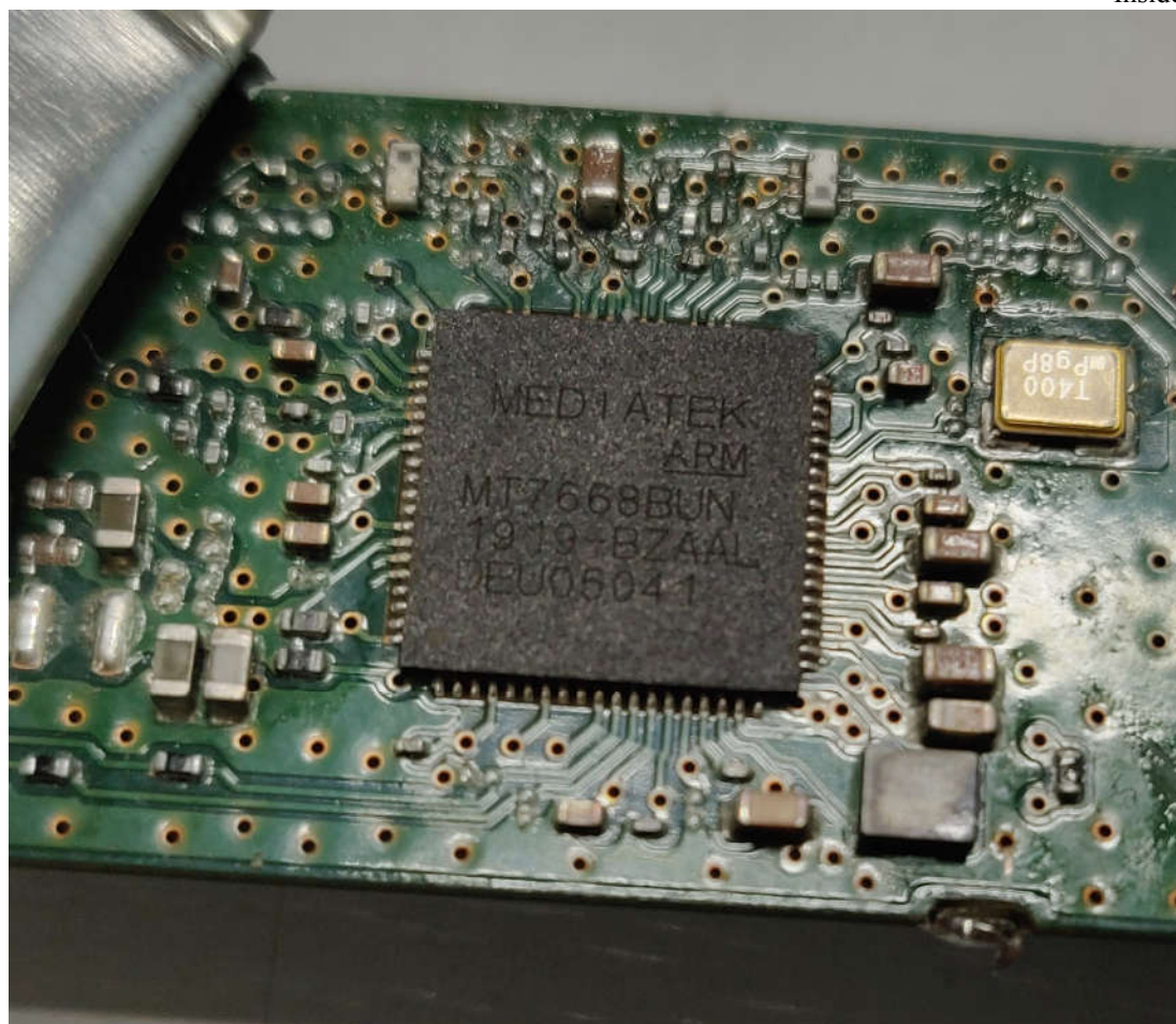
Figure 4 Inside of the EUT
