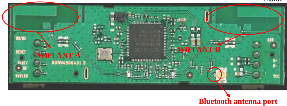
Figure 3 Inside of the EUT
