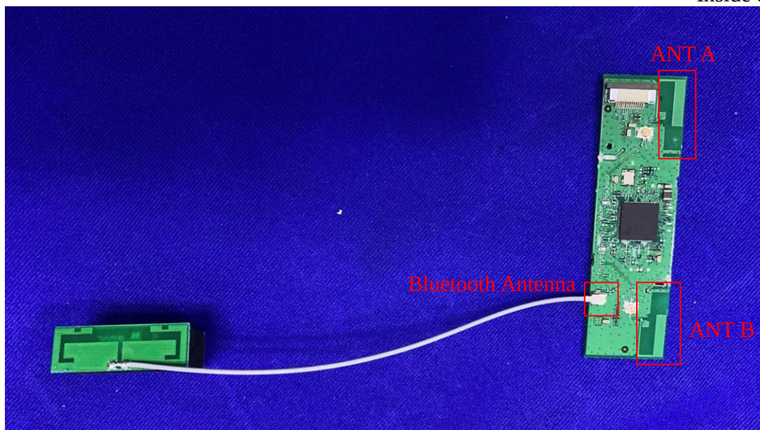
Figure 11 Inside of the EUT
