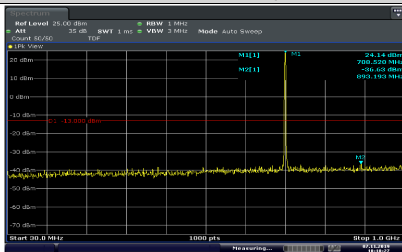
Band12-1.4MHz-QPSK-23095-6RB#0-Range1:30~1000MHz
