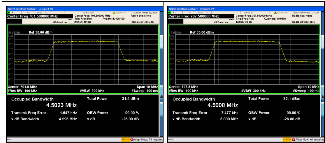
Band12-5MHz-QPSK-23035-25RB#0-PASS
