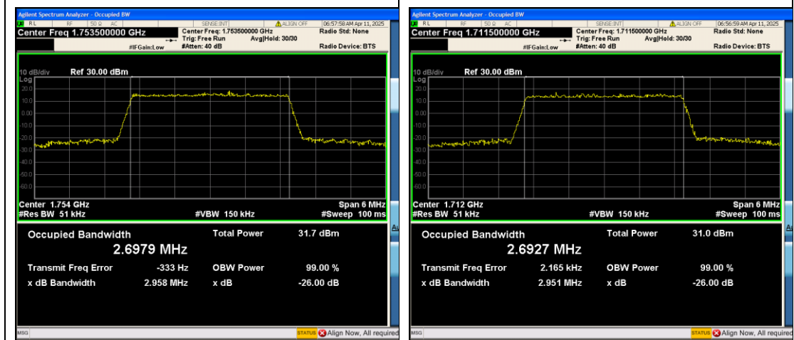
Band4-3MHz-QPSK-20385-15RB#0-PASS
