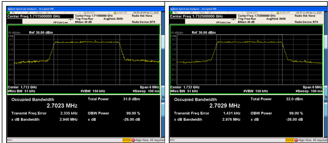
Band4-3MHz-QPSK-19965-15RB#0-PASS
