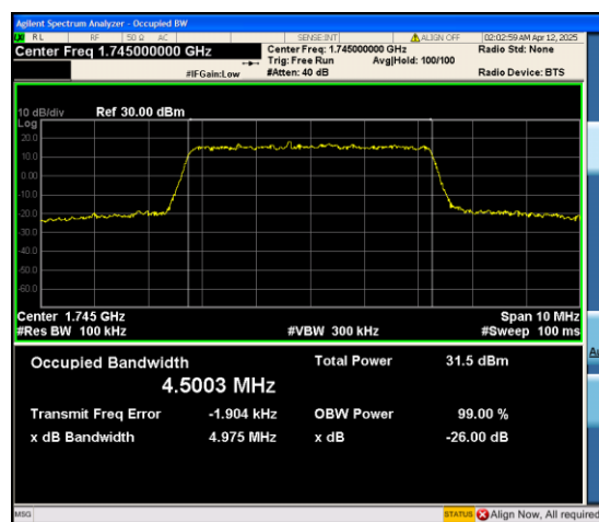
Band66-5MHz-16QAM-132322-25RB#0-PASS
