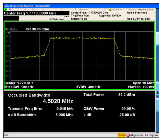
Band66-5MHz-QPSK-132647-25RB#0-PASS
