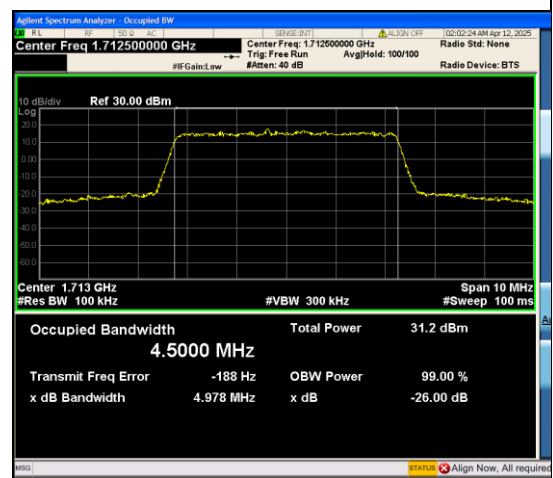
Band66-5MHz-16QAM-131997-25RB#0-PASS
