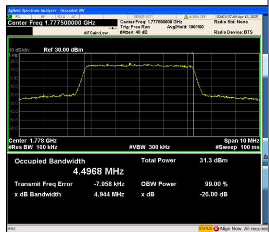
Band66-5MHz-16QAM-132647-25RB#0-PASS
