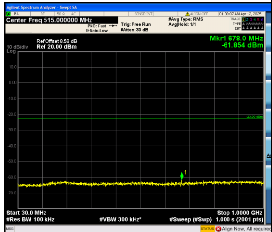
Band66_1.4MHz_QPSK_132322_6RB#0_30~1000_30~1000
