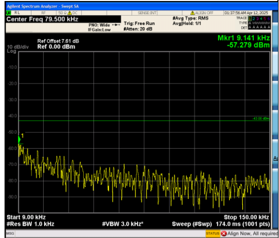
Band66_1.4MHz_QPSK_132322_6RB#0_0.009~0.15_0.009~0.15
