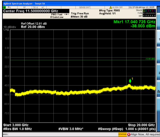
Band66_1.4MHz_QPSK_131979_6RB#0_3000~20000_3000~20000
