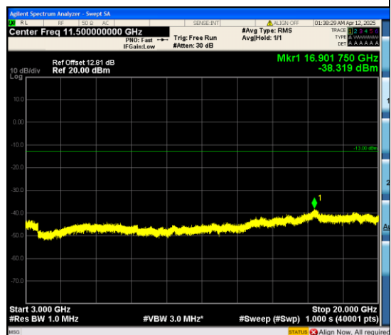
Band66_1.4MHz_QPSK_132322_6RB#0_3000~20000_3000~20000
