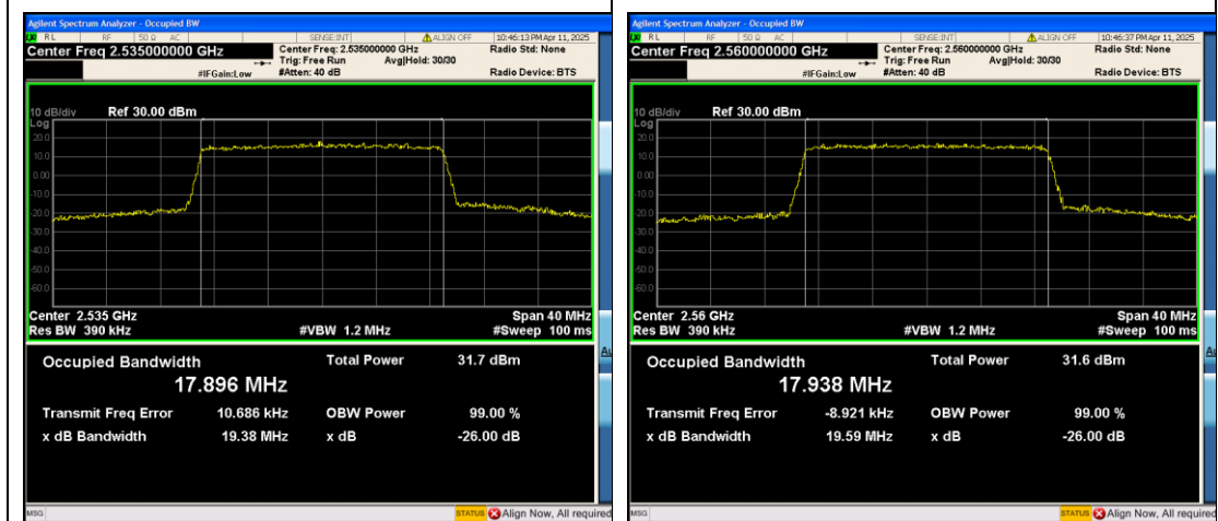
Band7-20MHz-16QAM-21100-100RB#0-PASS
