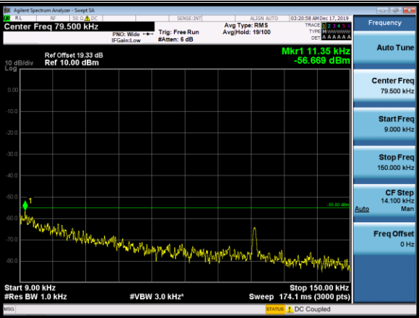
5MHz_MCH_QPSK_1RB#0
