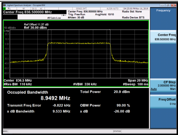
MCH_QPSK_50RB#0
