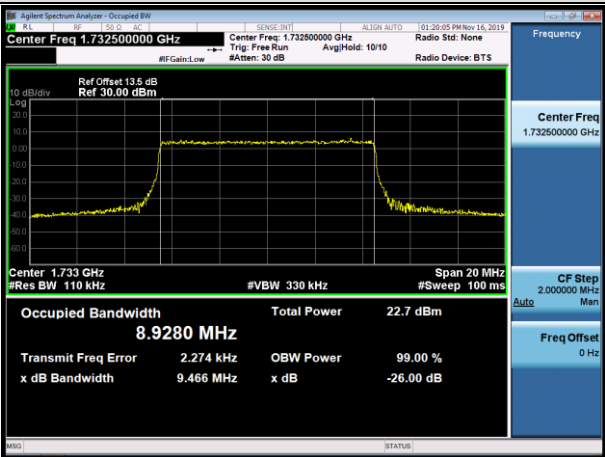
MCH_16QAM_50RB#0
