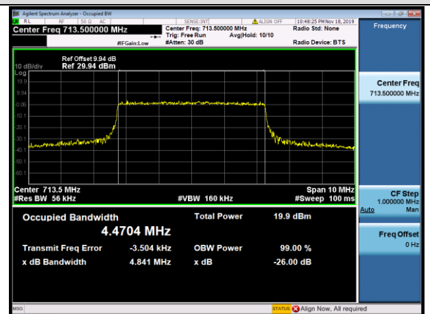
HCH_16QAM_25RB#0
