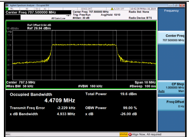
MCH_16QAM_25RB#0
