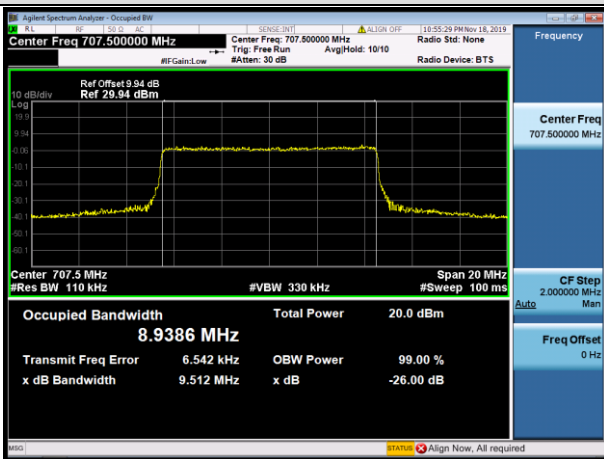
MCH_QPSK_50RB#0
