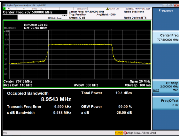
MCH_16QAM_50RB#0
