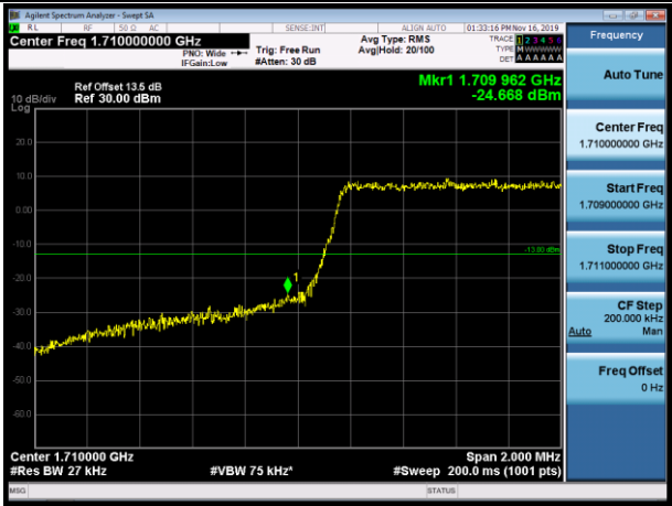
LCH_16QAM_6RB#0
