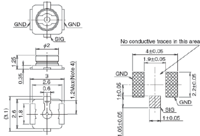
Figure 29: Dimensions of the UF.L-R-SMT Connector (Unit: mm)
