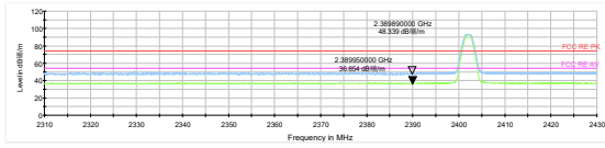
Bluetooth LE Channel 0 Peak+ Average
