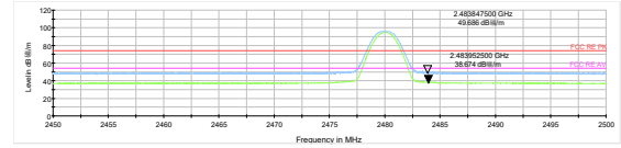
Bluetooth LE Channel 39 Peak+Average
