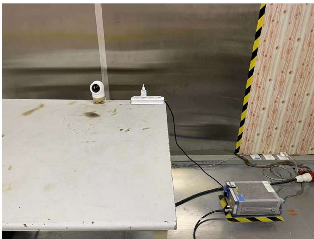
AC power conducted emission test:
