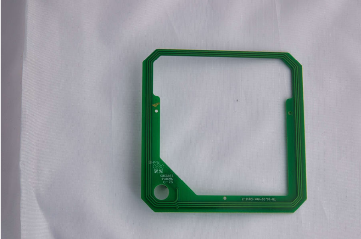
RFID Antenna PCB Top View
